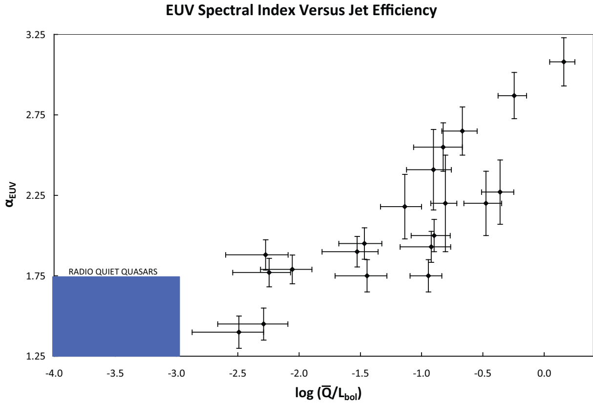
Fig. 1.— The correlation of \alpha_{\text{EUV}} versus the jet efficiency, \bar{Q}/L_{\text{bol}} (Punsly 2015b; Punsly and Marziani 2015). More powerful jets have depressed EUV emission.
