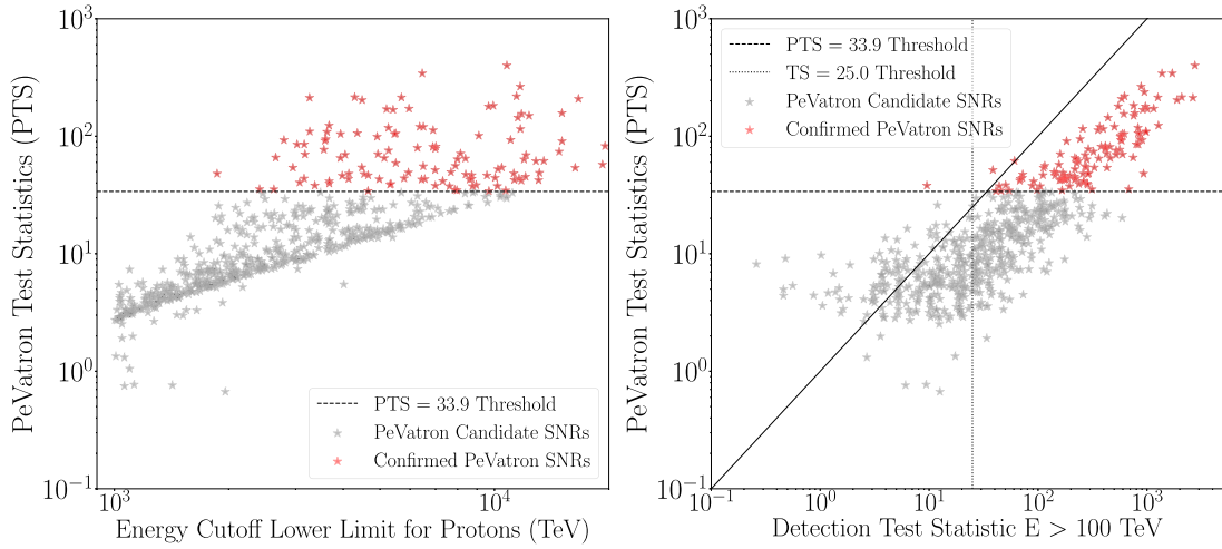
Fig. 8. Relation between the PTS and the lower 95% CL limit on the proton spectral cutoff (left) and detection test statistic, TS_{\text{Det}}^{100\text{TeV}} , of the \gamma -ray flux above 100 TeV (right), combining all \Gamma_p values between 2.0 and 2.3. Confirmed PeVatrons are marked in red and PeVatron candidates are marked in grey. The PTS threshold of 33.9, corresponding to a global 5\sigma significance for 100 independent tests, is indicated with horizontal dashed black lines. In the right panel, the vertical line indicates the \gamma -ray detection threshold TS_{\text{Det}}^{100\text{TeV}}=25 and the diagonal shows the equality PTS=TS_{\text{Det}} .
