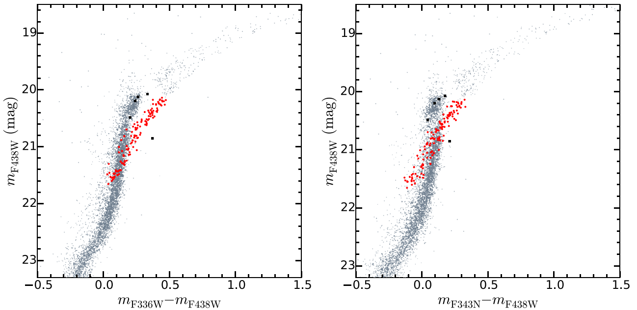
Figure 3. m_{F336W} - m_{F438W} versus m_{F438W} CMD (left-hand panel) and m_{F343N} - m_{F438W} versus m_{F438W} CMD (right-hand panel) of NGC 419. Red filled circles indicate the final RGB selected stars, while black filled squares represent the stars that did not pass the final selection.
