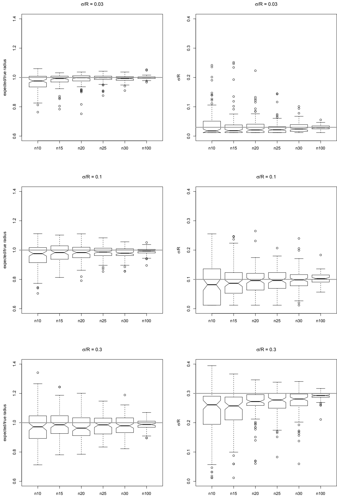
Fig. A.2. Box-and-whisker plots for the reconstructed \mathcal{R} and \sigma from 100 random realisations of the R \sin i distribution with no censoring and no truncation at different \sigma/\mathcal{R} values and different number of measurements per bin.
