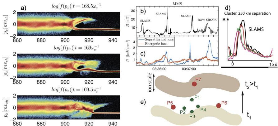
Fig. 4 Quasi-parallel shock. a Kinetic simulations of the time evolution of ion injection at a quasi-parallel shock with Mach number M=20 [18]. b, c MMS measurements of ion energization by SLAMS. d SLAMS evolution in Cluster data [23], e sketch illustrating the need for seven spacecraft to resolve spatio-temporal variations at SLAMS
