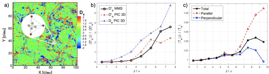
Fig. 8 Energy dissipation and particle energization in turbulence due to coherent structures. a spatial distribution of energy dissipation as seen in Particle-In-Cell simulations, showing that dissipation is concentrated at kinetic-scale coherent structures [94]. b simulations and MMS observations [90] showing that the strongest dissipation occurs in regions of highest current. c MMS measurements of electron heating showing that strong parallel electron heating is associated to dissipation and high currents
