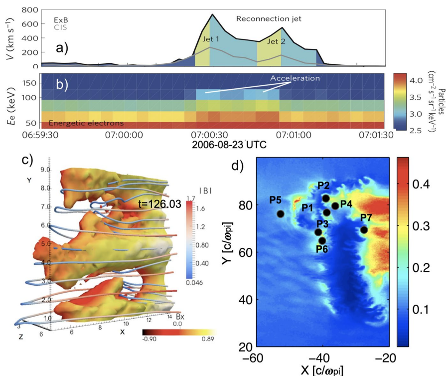
Fig. 10 Electron energization at jet fronts. In situ observations of reconnection jets: a plasma flow, b large-scale electron energization [134]. Numerical simulations showing nonlinear structures at jet fronts: c 3D isosurfaces of density with superimposed field lines from MHD simulations [150]. d parallel electron temperature from Particle-In-Cell simulations [151]. Schematic seven spacecraft constellation, P1–P7, would allow the spatial and temporal evolution of electron energization at jet fronts, as well as scale coupling, to be characterized
