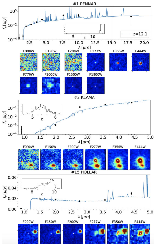
Figure 2. Photometry and best fit model of the galaxies #1 (top), #2 (middle), and #15 (bottom). The inset show the probability redshift distribution. We also report cutout images of the NIRCam/MIRI filters for the same galaxies, whose position is shown with a white cross.
