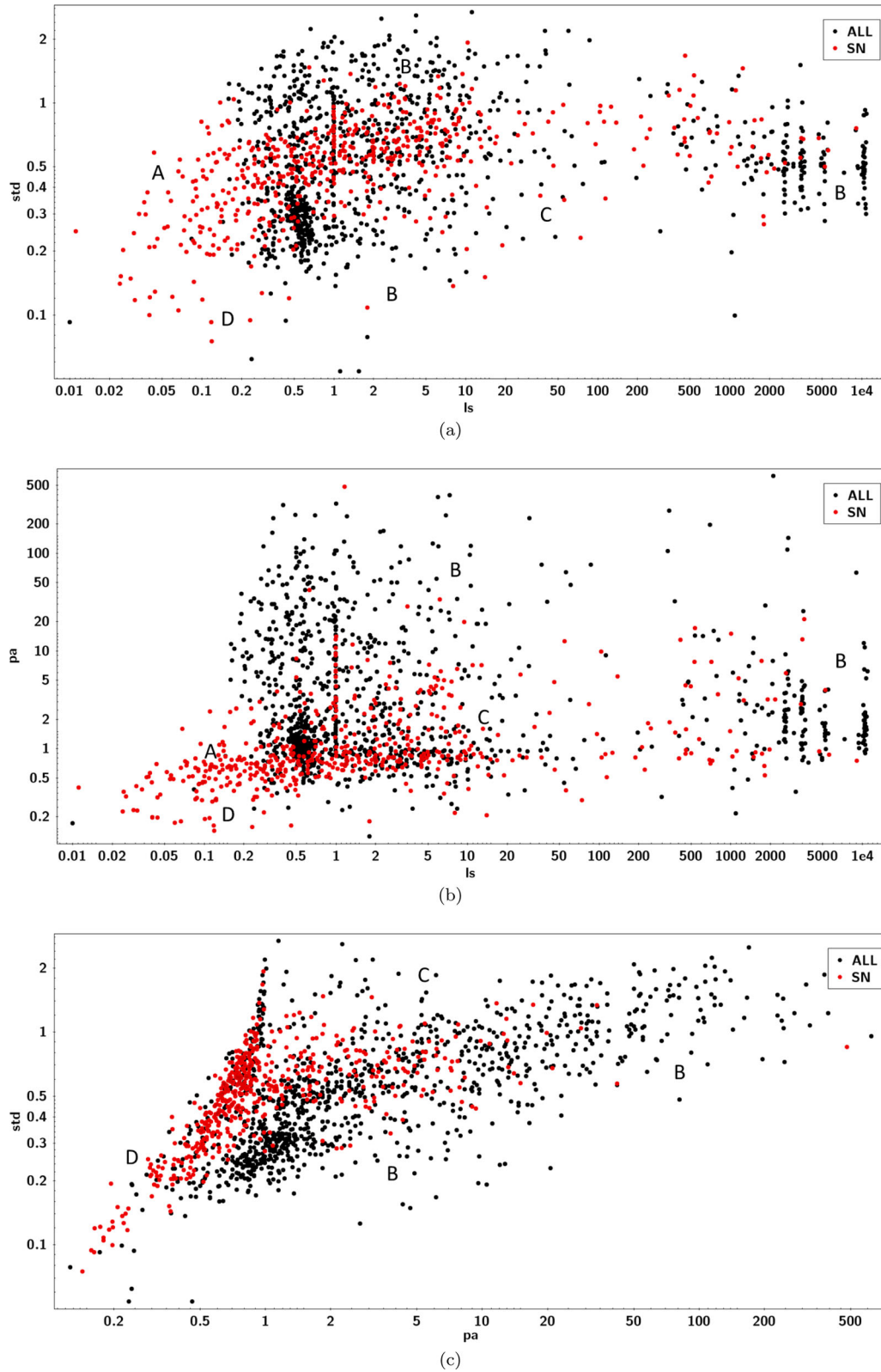
Figure 11. Panel (a): comparison of features std versus l_s in the case of SN versus ALL experiment; panel (b): the same plot but between pa and l_s features; panel (c): the same plot but between std and pa features. Red colour is related to SN objects and black to ALL class objects. The labels indicate, respectively, (A) pure SN region (i.e. a region populated only by SN objects), (B) sparse SN region (weak percentage of SN objects), (C) mixed zone and (D) almost pure SN region. The vertical structure at l_s = 1 is an effect introduced by the sampling frequency of the survey (the structure is mainly populated by AGN, BI and SN).
