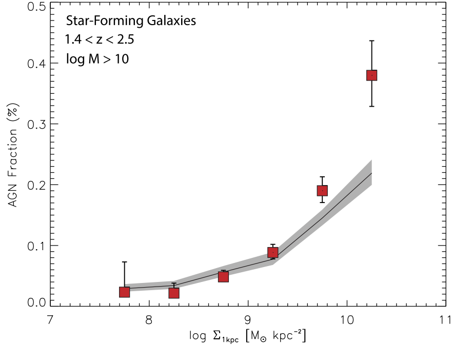
Figure 9. AGN fraction vs. \Sigma_{1 \text{ kpc}} for star-forming galaxies with M_* > 10^{10} M_\odot in the redshift range 1.4 < z < 2.5 . The black solid line shows the expected AGN fraction in galaxies matched in mass to those in the \Sigma_{1 \text{ kpc}} bins. Error bars and the gray shaded region show the 68.3% binomial confidence limits. At the highest values of \Sigma_{1 \text{ kpc}} , we find that the AGN fraction exceeds what we expect in a mass-matched control sample, suggesting that the increased nuclear activity in these galaxies is linked to their high core density.
