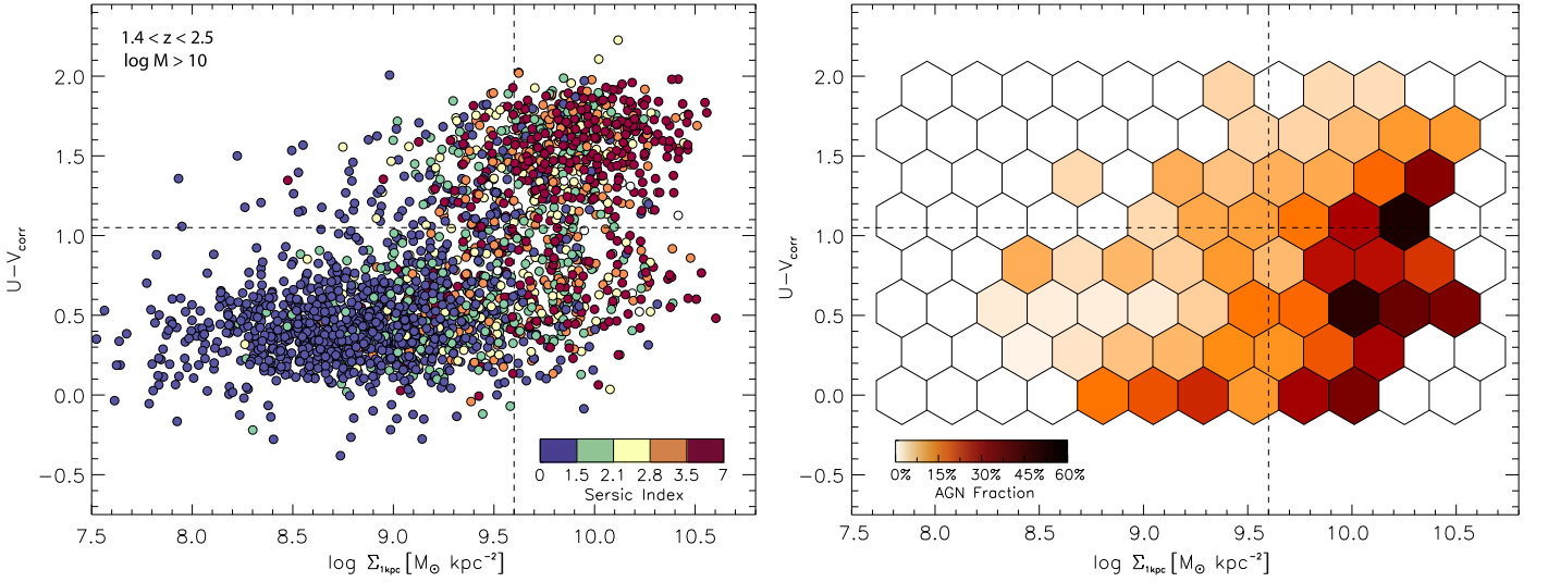
Figure 8. (Left) Central surface mass density ( \Sigma_{1 \text{ kpc}} ) vs. rest-frame color for galaxies with M_* > 10^{10} M_\odot in the redshift range 1.4 < z < 2.5 . Points are color-coded by their best-fit Sérsic index. (Right) AGN fraction in regions of \Sigma_{1 \text{ kpc}} -color space. We find that the AGN fraction peaks among the compact, star-forming population; a result that holds true whether compact galaxies are defined using \Sigma_e or \Sigma_{1 \text{ kpc}} .
