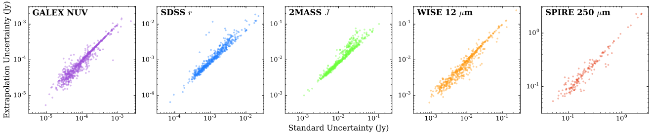
Fig. 9. Plots showing how uncertainty estimates determined the standard way (with full-size randomly generated sky apertures; see Sect. 3.7) compare to uncertainty estimates determined using the aperture noise extrapolation technique described in Sect. 3.8, for various bands.
