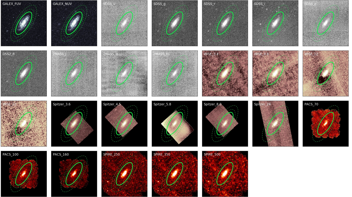
Fig. 6. Photometry thumbnail image grid for NGC 4559. CAAPR produces an image like this for every source. Solid lines show master aperture, whilst dashed lines demark background annulus. Several of the fluxes for NGC 4559 have flags (flags are defined in Sect. 4). WISE 12 \mu\text{m} flux has “A” flag due to negative flux artefact in master aperture, whilst WISE 22 \mu\text{m} flux has “a” flag, due to a less pronounced version of the same feature. The Spitzer 3.6, 4.5, 5.8, and 8.0 \mu\text{m} fluxes have “N” flags (although these are borderline cases), as <40% of pixels in their sky annuli have coverage, so it is assumed that any background estimate will be unreliable (similarly, the lack of coverage in their master apertures would, independently, warrant “n” flags). Spitzer 24 \mu\text{m} and PACS 70, 100, and 160 \mu\text{m} fluxes have “n” flags, as <80% of pixels in their sky annuli have coverage, potentially reducing reliability of background estimate.
