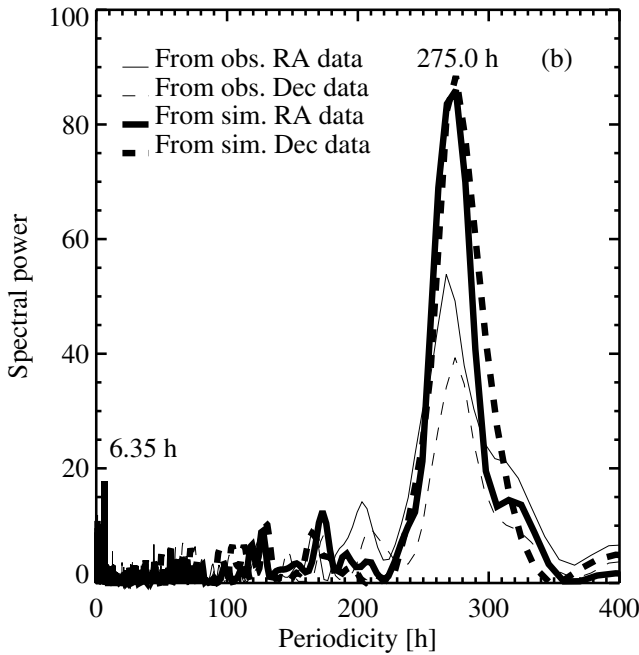
Fig. 10. Simulation with the highest K-S probability from the comparison of RA coordinate distributions. a) As previously, bullets ( \bullet ) show the observationally derived spin axis (Fig. 2). Diamonds ( \blacklozenge ) correspond to the simulated spin axis orientation of a body with 1:1.90:2.84, and E_l = 6.7 \times 10^{-5} when an averaging of 10 h and a uniformly distributed random noise with an amplitude of 0.03^\circ have been considered. b) (Thick lines) Lomb periodograms of the RA and Dec simulated data (diamonds shown in Fig. 10a). The Lomb periodograms of the observationally derived coordinates (Fig. 3) have also been included (with thin lines).
