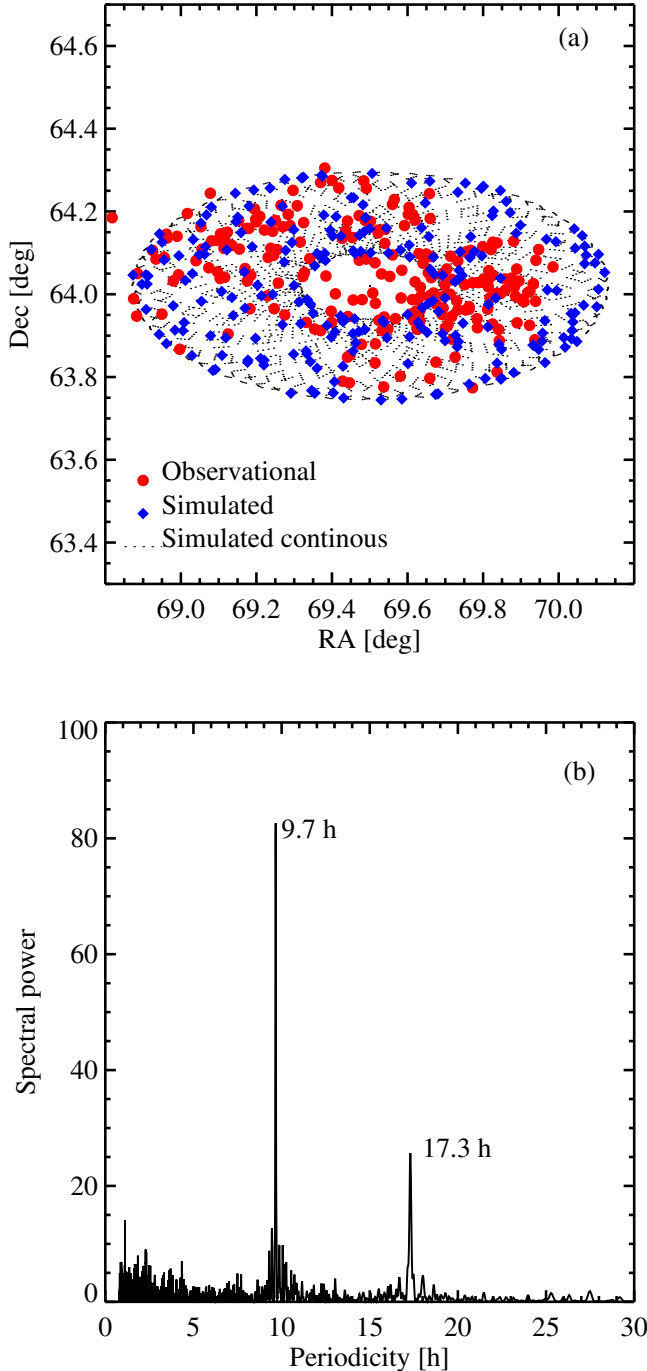
Fig. 5. a) Bullets (•) show the spin axis orientation as determined with the SPC method (Fig. 2). Small dots (•) are the spin vector orientation for a simulated body with inertia moments equal to those derived from the shape of 67P assuming homogeneity, and an E_I = 1.9 \times 10^{-6} under case 1 circumstances. These data are displayed with a time separation of 1 h. Diamonds (◆), to be compared with the bullet distribution, correspond to the orientation of the spin axis for the simulation performed at the time and date associated with each determination made with the SPC method. To locate the diamonds, neither noise nor averaging have been included. b) Lomb periodogram of the Dec-simulated coordinates (diamonds) shown in Fig. 5a. The RA coordinate periodogram is exactly the same as that of the Dec data, only small differences in spectral power (height of the peak) can be appreciated.
