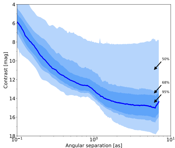
Fig. 22: Median 5\sigma contrast achieved by IRDIS in DBI H23 mode (H2 ADI only) in 1h30 observing time on average with T-LOCI post-processing. The plain blue line represents the median, and the different shades of blue background represent the 95%, 68% and 50% completeness intervals.
