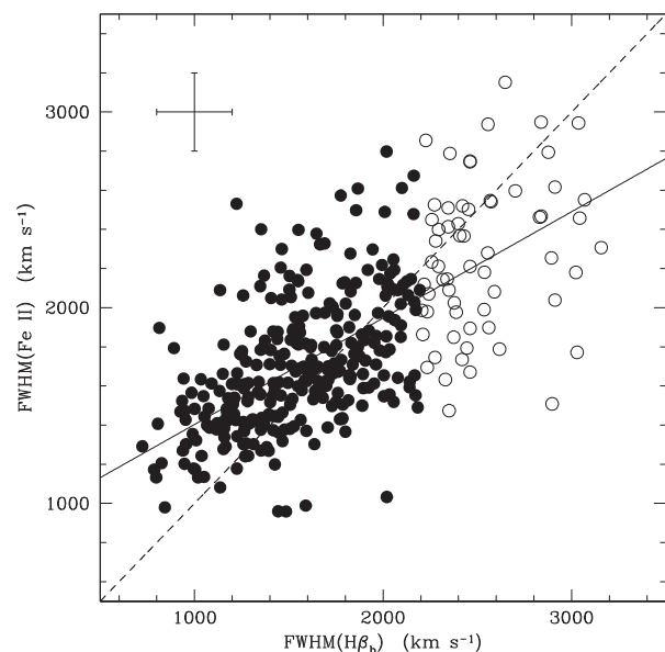
Figure 12. The FWHM of \text{H}\beta_b plotted against the FWHM of Fe II. The solid line is the best fitting, the dashed line is the 1:1 relation. Symbols are the same as in Fig. 5.
