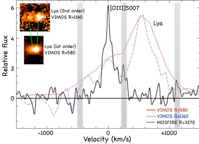
Fig. 9. Velocity profiles of [O III] \lambda 5007 and Ly \alpha lines relative to systemic. The [O III] \lambda 5007 line is shown in black, the Ly \alpha first order in red, and the Ly \alpha second order with the dashed blue line. The positions and widths of the sky lines are indicated by gray stripes.
