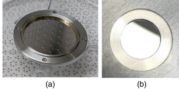
Fig. 1 Sample filters with a thin PI membrane, coated with Al. (a) Filter sample with a 5-mm pitch Au-plated SS honeycomb mesh mounted on a TF130 standard frame. (b) Meshless filter sample mounted on a TF110 standard frame, as used in the campaigns here reported.
