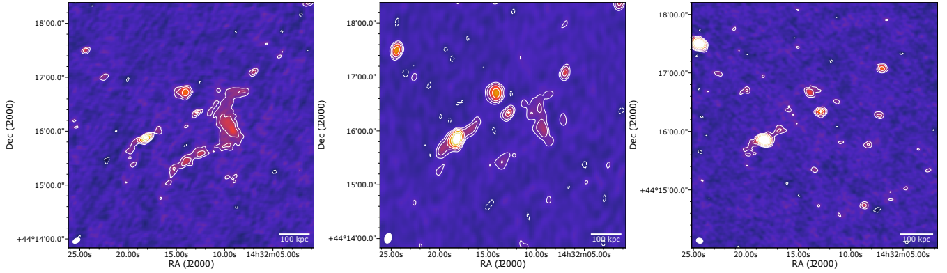
Figure 2. Left: LOFAR HBA 120-168 MHz image. Contour levels are drawn at [-/+3, 6, 12, 24] \times \sigma ( \sigma = 180 \mu\text{Jy/beam} ) and the restoring beam of 5.0 \times 8.7'' is shown by the ellipse in the lower-left corner. Middle: GMRT 325 MHz image. Contour levels are drawn at [-/+3, 6, 12, 24] \times \sigma ( \sigma = 55 \mu\text{Jy/beam} ); the restoring beam is 7.5 \times 11.6'' . Right: VLA 1-2 GHz B+C array image. Contour levels are drawn at [-/+3, 6, 12, 24] \times \sigma ( \sigma = 18 \mu\text{Jy/beam} ); the restoring beam is 5.2 \times 7.0'' . The cross marks the location of the BCG. No emission from the extended LOFAR source is detected in the VLA image.
