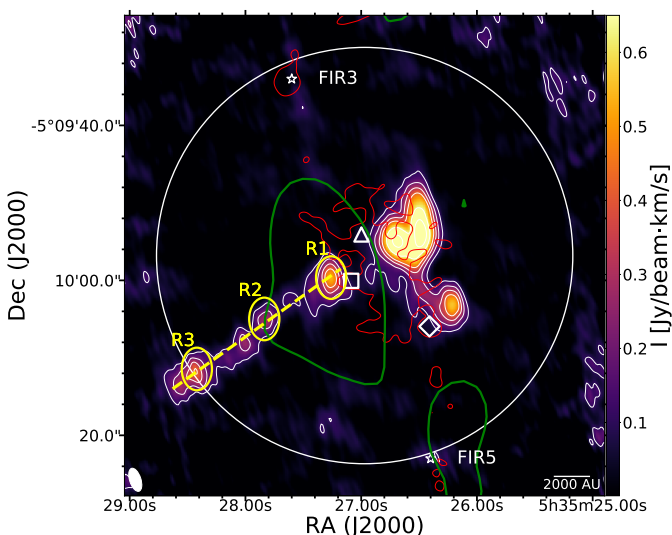
Fig. 1. Integrated intensity (between -18 and 43 km s^{-1} ) map of the SiO ( J = 2-1 ) emission towards OMC-2 FIR4; white contours are 10%, 20%, 30%, 40%, 60%, and 80% of the maximum value ( 0.985 Jy/beam-km s^{-1} ). The velocity channels were selected in the emission map with a 5\sigma cut-off around the emission peak ( 1\sigma = 6.7 \times 10^{-4} Jy/beam). Red contour indicates the 10\sigma of the 85 GHz continuum emission (Neri et al. in preparation; \sigma = 3.8 \times 10^{-5} Jy/beam). Green contour is the 7.5\sigma integrated emission of \text{HC}_5\text{N} described in Fontani et al. (2017), with 1\sigma = 3.6 \times 10^{-3} Jy/beam-km s^{-1} . This region, with an average radius of \sim 5000 AU, is also where Fontani et al. (2017) inferred the CR ionisation rate of \zeta = 4 \times 10^{-14} s^{-1} . The yellow open ellipses along the jet represent the three regions used to extract the spectra shown in Fig. 2 and are labelled R1, R2, and R3, while the yellow dashed line encompassing these three regions shows the cut used to generate the PV plot in Fig. 3. The three main protostars in FIR4, namely HOPS-108 (RA(J2000) = 05^{\text{h}}35^{\text{m}}27^{\text{s}}.086 , DEC(J2000) = -05^{\circ}10'00''.06 ), HOPS-64 (RA(J2000) = 05^{\text{h}}35^{\text{m}}26^{\text{s}}.998 , DEC(J2000) = -05^{\circ}09'54''.08 ), and VLA15 (RA(J2000) = 05^{\text{h}}35^{\text{m}}26^{\text{s}}.41 , DEC(J2000) = -05^{\circ}10'05''.94 ) (Tobin et al. 2019), are represented by the three open symbols: square, triangle, and diamond, respectively. The white open circle marks the primary beam Full Width Half Maximum (FWHM) for the NOEMA observations. The bottom left ellipse represents the synchrotron emission.
