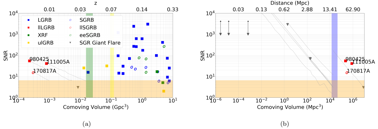
Fig. 7 ECLAIRs on-axis count SNR for transients in our sample. The orange horizontal band represents the detection limit of ECLAIRs at \text{SNR} = 6.5 . (a) On-axis count SNR obtained for the local GRBs. The green and yellow bands represent the O4 LIGO distance sensitivity limits for NS-NS and BH-NS mergers respectively. The light grey trails represent the evolution of the on-axis count SNR with the redshift. (b) On-axis SNR calculated for the SGR Giant Flares. The blue band represents the approximate distance from the Virgo Cluster. GF 790205, GF 980827 and GF 041227 on the top left have SNR over 10^4 and would most likely saturate the instrument, we show them with arrows to improve the readability of the graph.
