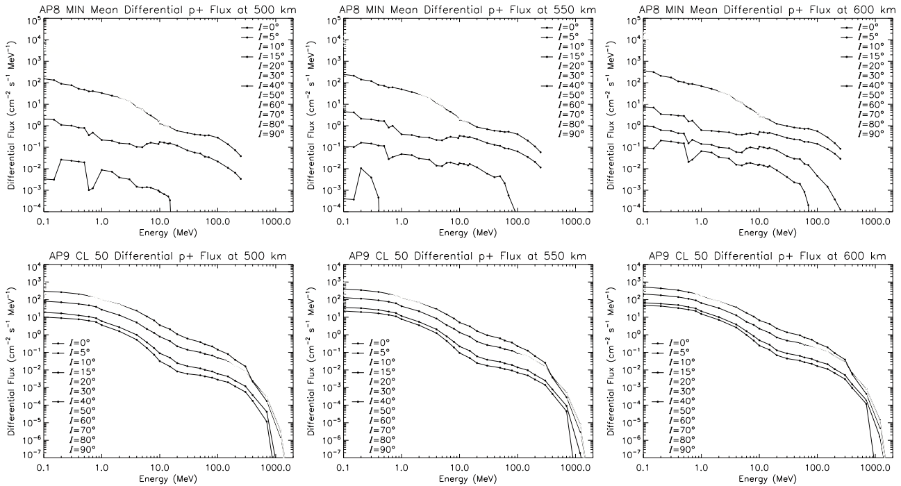
Figure 4. Orbit averaged differential fluxes of trapped protons for mean AP8 MIN (top panels) and AP9 50% CL (bottom panels) models computed for altitudes 500, 550 and 600km altitudes, respectively, from left to right and for different orbital inclinations I .
