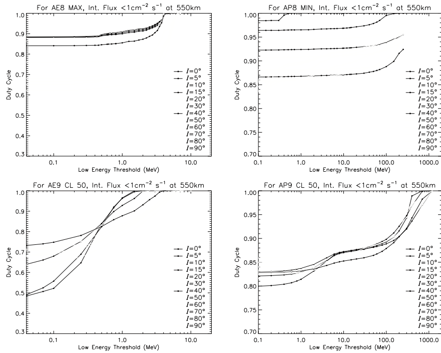
Figure 9. Duty cycle for particle flux < 1 \text{ cm}^{-2} \text{ s}^{-1} for different orbital inclination as a function of the low-energy threshold for AE8MAX (top left), AE9 50% CL (bottom left) models of trapped e^- and AP8MIN (top right), AP9 50% CL (bottom right) models of trapped p^+ .
