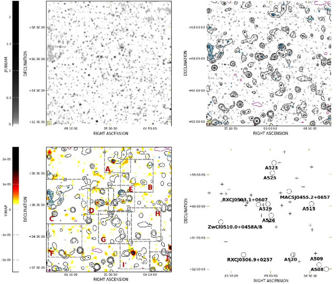
Figure 6. Top left panel: SRT+NVSS image in colours (FWHM 3.5'). Top right panel: contours of the SRT image (-60 mJy/beam, 60 mJy/beam, 150 mJy/beam, 500 mJy/beam, negative in magenta and positive in black; resolution 13.9' \times 12.4' ) and of the SRT+NVSS image after compact sources subtraction (starting at 3\sigma and increasing by a factor \sqrt{2} , in blue; \sigma=2.5 mJy/beam, resolution 3.5' \times 3.5' ) overlaid on the SRT+NVSS image in colours (FWHM 3.5'). Bottom left panel: SRT and SRT+NVSS after point-source subtraction in contours overlaid on the Planck Y-map (see text) in colours. The contours from SRT and from the residual SRT+NVSS image are the same as in the top right panel. The resolution of the Planck Y-map is 10' . Dots indicate the position of clusters with redshift identification (see Table 1), while crosses indicate clusters without redshift identification (see Table 2). Bottom right panel: Location of clusters with known redshift (circles and labels) and of the sources discussed in this paper (crosses), see Table 5.
