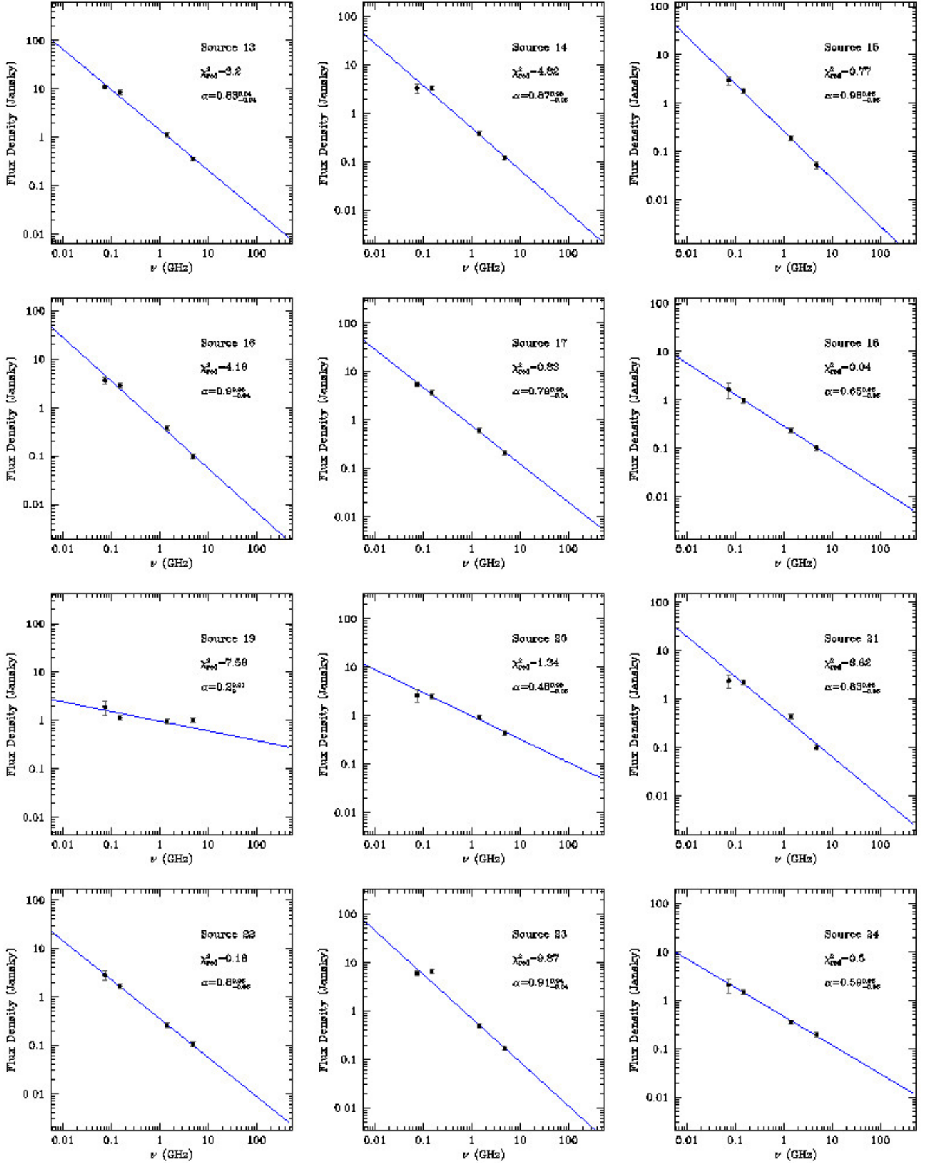
Figure A3. Flux density versus frequency for the last 12 sources in the catalogue. For each source the flux density as measured by VLSSr, TGSS, combined SRT+NVSS, and GB6 images is shown along with the power law fit, the resulting spectral index \alpha value and the \chi^2_{\text{red}} of the fit.
