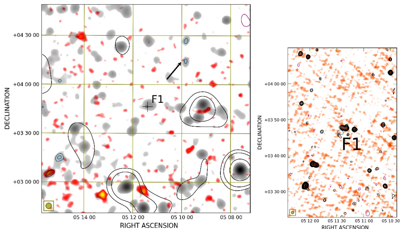
Figure 13. Region F. Left panel: SRT contours ( -60 mJy/beam, 60 mJy/beam, 150 mJy/beam, 500 mJy/beam, negative in magenta and positive in black; resolution 13.9' \times 12.4' ) and SRT+NVSS after compact sources subtraction contours (in blue, starting from 3\sigma and the remaining increasing by a factor \sqrt{2} ; \sigma=2.5 mJy/beam, resolution 3.5' \times 3.5' ) overlaid on X-ray emission from the RASS in red colours and radio emission from the SRT+NVSS (resolution 3.5' ) in gray colours. Right panel: NVSS contours -3\sigma (magenta, \sigma=0.45 mJy/beam), 3\sigma , and increasing by a factor \sqrt{2} (black) overlaid on the TGSS in colours. The black arrow marks the position of the candidate giant radio galaxy we found (see § B). The colorbars are the same as in Fig. 7.
