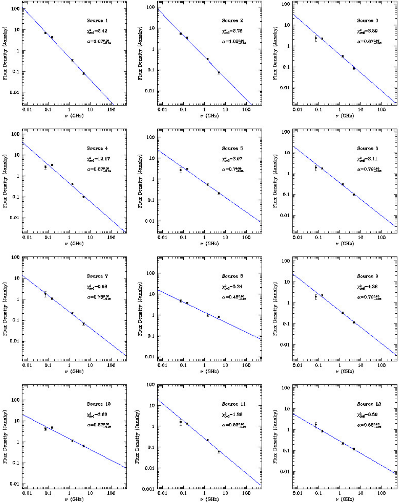
Figure A2. Flux density versus frequency for the first 12 sources in the catalogue. For each source the flux density as measured by VLSSr, TGSS, combined SRT+NVSS, and GB6 images is shown along with the power law fit, the resulting spectral index \alpha value and the \chi^2_{\text{red}} of the fit.
