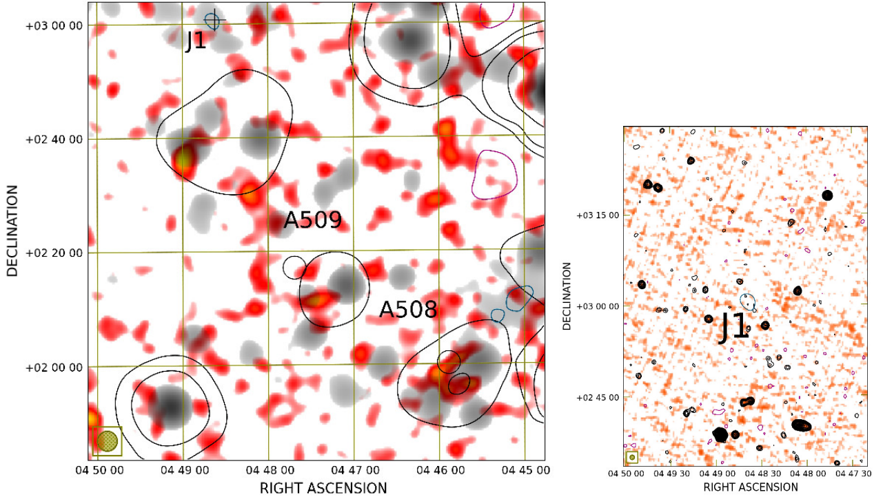
Figure 17. Region J. Left panel: SRT contours ( -60 mJy/beam, 60 mJy/beam, 150 mJy/beam, 500 mJy/beam, negative in magenta and positive in black; resolution 13.9' \times 12.4' ) and SRT+NVSS after compact sources subtraction contours (in blue, starting from 3\sigma and the remaining increasing by a factor \sqrt{2} ; \sigma=2.5 mJy/beam, resolution 3.5' \times 3.5' ) overlaid on X-ray emission from the RASS in red colours and radio emission from the SRT+NVSS (resolution 3.5' ) in gray colours. Right panel: NVSS contours -3\sigma (magenta, \sigma=0.45 mJy/beam), 3\sigma , and increasing by a factor \sqrt{2} (black) overlaid on the TGSS in colours. The colorbars are the same as in Fig. 7.
