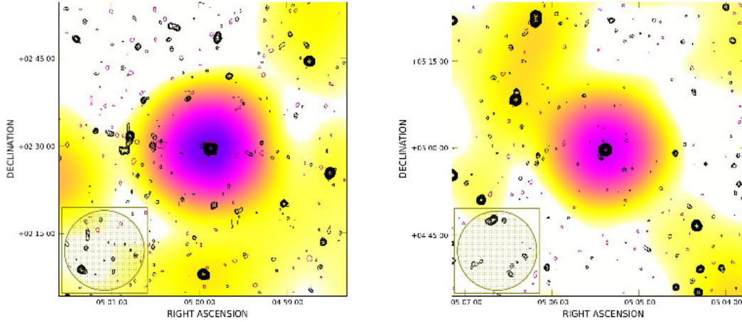
Figure 3. Sources used for the beam measurement (left panel) and for the comparison of the NVSS and SRT flux density scales (right panel). The SRT image in the same frequency range as the NVSS is shown in colours, while the NVSS emission is shown in contours. The contour levels are -1.35, 1.35 mJy/beam (with a beam of 45'' ) and increase by a factor \sqrt{2} , positive contours shown in black and negative contours shown in magenta. The beam in the bottom left corner represents the SRT spatial resolution of 13.66' as found in § 3.1. The colorbar is the same as Fig. 2.
