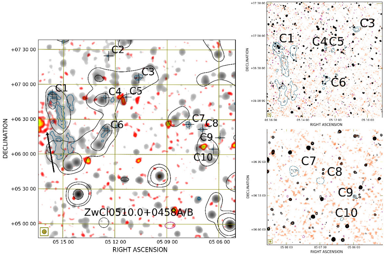
Figure 10. Region C. Left panel: SRT contours ( -60 mJy/beam, 60 mJy/beam, 150 mJy/beam, 500 mJy/beam, negative in magenta and positive in black; resolution 13.9' \times 12.4' ) and SRT+NVSS after compact sources subtraction contours (in blue, starting from 3\sigma and the remaining increasing by a factor \sqrt{2} ; \sigma=2.5 mJy/beam, resolution 3.5' \times 3.5' ) overlaid on X-ray emission from the RASS in red colours and radio emission from the SRT+NVSS (resolution 3.5' ) in gray colours. Right panels: NVSS contours -3\sigma (magenta, \sigma=0.45 mJy/beam), 3\sigma , and increasing by a factor \sqrt{2} (black) overlaid on the TGSS in colours. The black arrow marks the position of A539. The colorbars are the same as in Fig. 7.
