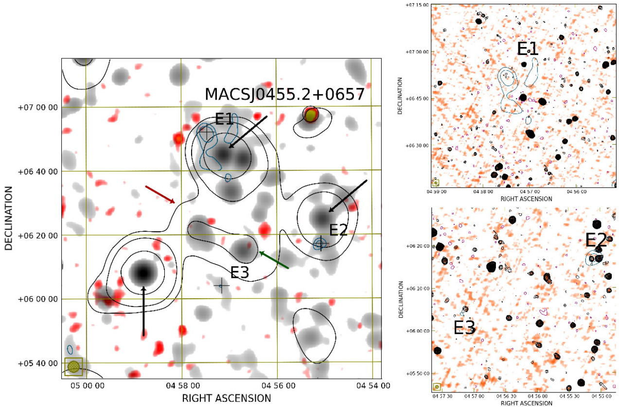
Figure 12. Region E. Left panel: SRT contours ( -60 mJy/beam, 60 mJy/beam, 150 mJy/beam, 500 mJy/beam, negative in magenta and positive in black; resolution 13.9' \times 12.4' ) and SRT+NVSS after compact sources subtraction contours (in blue, starting from 3\sigma and the remaining increasing by a factor \sqrt{2} ; \sigma=2.5 mJy/beam, resolution 3.5' \times 3.5' ) overlaid on X-ray emission from the RASS in red colours and radio emission from the SRT+NVSS (resolution 3.5' ) in gray colours. Right panels: NVSS contours -3\sigma (magenta, \sigma=0.45 mJy/beam), 3\sigma , and increasing by a factor \sqrt{2} (black) overlaid on the TGSS in colours. The black arrows mark the position of 4C +06.21, PKS 0456+060, and LQAC 073+006 001, and the red arrow the faint large-scale emission SRT emission in between these three bright compact sources. The green arrow marks the location where signal is clearly visible in the SZ and X-ray images while in the SRT+NVSS after compact sources subtraction is detected only with a 2\sigma significance. The colorbars are the same as in Fig. 7.
