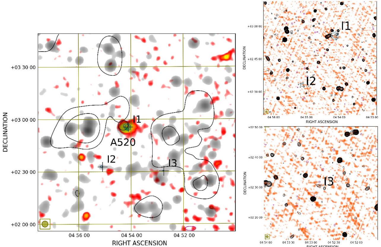
Figure 16. Region I. Left panel: SRT contours ( -60 mJy/beam, 60 mJy/beam, 150 mJy/beam, 500 mJy/beam, negative in magenta and positive in black; resolution 13.9' \times 12.4' ) and SRT+NVSS after compact sources subtraction contours (in blue, starting from 3\sigma and the remaining increasing by a factor \sqrt{2} ; \sigma=2.5 mJy/beam, resolution 3.5' \times 3.5' ) overlaid on X-ray emission from the RASS in red colours and radio emission from the SRT+NVSS (resolution 3.5' ) in gray colours. Right panels: NVSS contours -3\sigma (magenta, \sigma=0.45 mJy/beam), 3\sigma , and increasing by a factor \sqrt{2} (black) overlaid on the TGSS in colours. The colorbars are the same as in Fig. 7.
