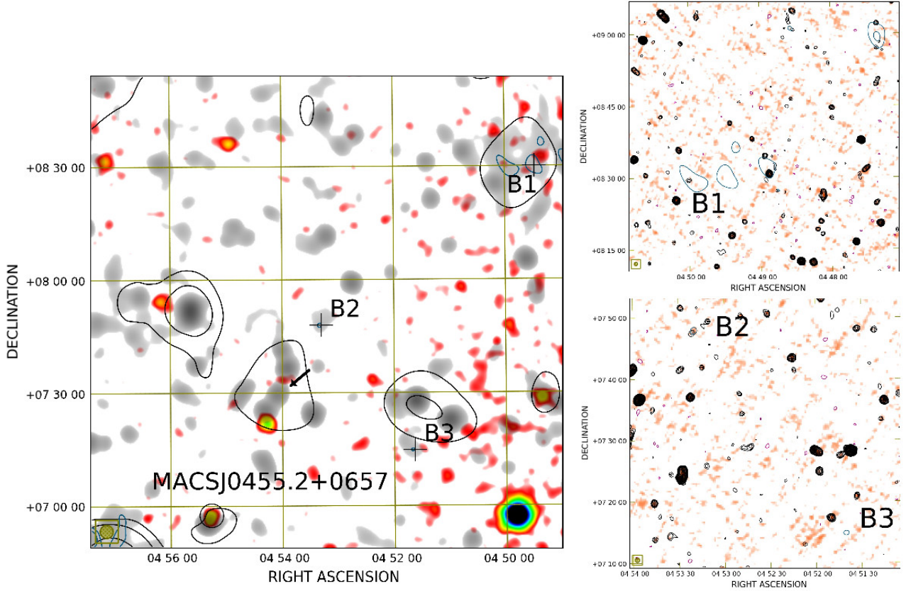
Figure 8. Region B. Left panel: SRT contours ( -60 mJy/beam, 60 mJy/beam, 150 mJy/beam, 500 mJy/beam, negative in magenta and positive in black; resolution 13.9' \times 12.4' ) and SRT+NVSS after compact sources subtraction contours (in blue, starting from 3\sigma and the remaining increasing by a factor \sqrt{2} ; \sigma=2.5 mJy/beam, resolution 3.5' \times 3.5' ) overlaid on X-ray emission from the RASS in red colours and radio emission from the SRT+NVSS (resolution 3.5' ) in gray colours. Right panels: NVSS contours -3\sigma (magenta, \sigma=0.45 mJy/beam), 3\sigma , and increasing by a factor \sqrt{2} (black) overlaid on the TGSS in colours. The black arrow marks the region shown in the zoom of Fig. 9. The colorbars are the same as in Fig. 7.
