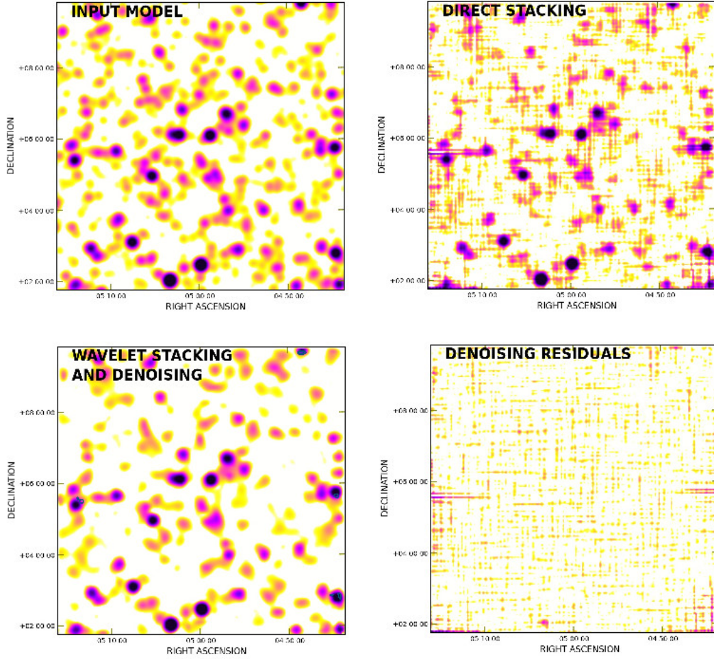
Figure C2. Top-left panel: model of the sky including only the point-like sources. Top-right panel: the image derived by direct averaging all the RA and DEC baseline subtracted scans. Bottom-left panel: image after applying the wavelet stacking and denoising algorithms. The blue contours represent the difference between the wavelet stacking and denoising image and the input model and start from 3\sigma of the first. Bottom-right panel: difference of the last two panels.
