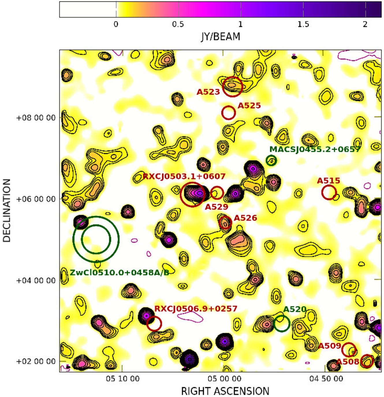
Figure 2. SRT image in colours and contours in the frequency range 1.3-1.8 GHz. The contours are -3\sigma , 3\sigma ( \sigma = 20 mJy/beam) and the remaining scale by a factor \sqrt{2} . Negative contours are represented in magenta, while positive contours are in black. The angular resolution of the images is 13.9' \times 12.4' and BPA = -58.5^\circ at the center of the observing band. The circles and labels identify the position of the galaxy clusters in the field of view with known redshift. The size of the circles is proportional to R_{200} of the corresponding clusters (see Table 4), large circles are close-by clusters while small circles are distance clusters. For systems with an upper limit for R_{200} , we used the value of the upper limit. We highlight in red clusters with redshift between 0.08 and 0.15, in green clusters with redshift outside this range.
