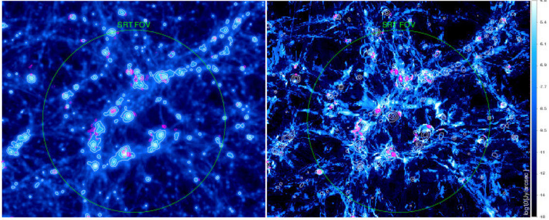
Figure 21. Left panel: estimated virial volume of all halos in the box (based on their total matter density, white contours) and detectable radio emission in the SRT observing configuration presented in this paper (purple contours) overlaid on the projected gas density (colours). Right panel: the colours show the projected full radio emission at the nominal resolution of the simulation (83 kpc/cell) and assuming this field is at z = 0.1 . The contours are the same as in the left panel. The green circles in both images represent the field of view of SRT if the simulated volume is located at z = 0.1 .
