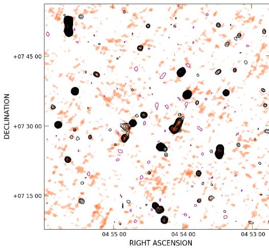
Figure 9. Zoom of the central portion of Region B (see arrow in Fig. 8). The image shows the NVSS contours ( -1.35 mJy/beam, 1.35 mJy/beam, and the remaining scaled by a factor \sqrt{2} , negative in magenta and positive in black) overlaid on the TGSS colours. The colorbar is the same as in the right panels of Fig. 7.
