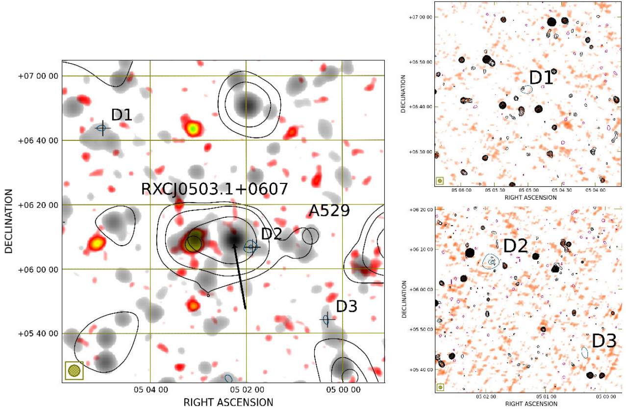
Figure 11. Region D. Left panel: SRT contours ( -60 mJy/beam, 60 mJy/beam, 150 mJy/beam, 500 mJy/beam, negative in magenta and positive in black; resolution 13.9' \times 12.4' ) and SRT+NVSS after compact sources subtraction contours (in blue, starting from 3\sigma and the remaining increasing by a factor \sqrt{2} ; \sigma=2.5 mJy/beam, resolution 3.5' \times 3.5' ) overlaid on X-ray emission from the RASS in red colours and radio emission from the SRT+NVSS (resolution 3.5' ) in gray colours. Right panels: NVSS contours -3\sigma (magenta, \sigma=0.45 mJy/beam), 3\sigma , and increasing by a factor \sqrt{2} (black) overlaid on the TGSS in colours. The black arrow marks the position of the quasar PKS 0459+060. The colorbars are the same as in Fig. 7.
