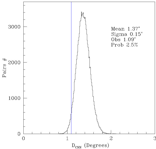
Figure 20. Distribution of D_{\text{CNN}} for the random sets of sources (black histogram). The histogram is well described by a Gaussian distribution with mean 1.37^\circ and standard deviation 0.15^\circ . The D_{\text{CNN}} for our sample is shown by the blue line.
