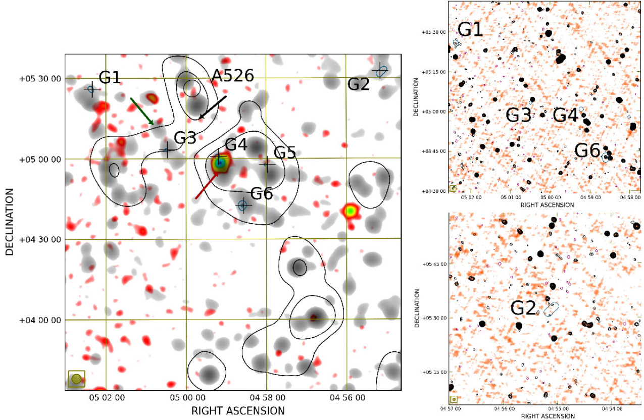
Figure 14. Region G. Left panel: SRT contours ( -60 mJy/beam, 60 mJy/beam, 150 mJy/beam, 500 mJy/beam, negative in magenta and positive in black; resolution 13.9' \times 12.4' ) and SRT+NVSS after compact sources subtraction contours (in blue, starting from 3\sigma and the remaining increasing by a factor \sqrt{2} ; \sigma=2.5 mJy/beam, resolution 3.5' \times 3.5' ) overlaid on X-ray emission from the RASS in red colours and radio emission from the SRT+NVSS (resolution 3.5' ) in gray colours. Right panels: NVSS contours -3\sigma (magenta, \sigma=0.45 mJy/beam), 3\sigma , and increasing by a factor \sqrt{2} (black) overlaid on the TGSS in colours. The black and red arrow mark respectively the locations of the galaxy cluster ZwCl0457.0+0511 and of the compact source PMN J0459+0455, while the green arrow a bridge of radio emission detected by SRT. The colorbars are the same as in Fig. 7.
