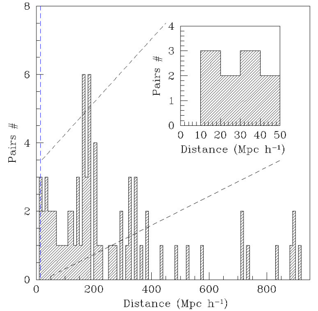
Figure 5. Distribution of 3-d distances between all the pairs of clusters with known redshift in the field. The dashed vertical blue line marks a 3-d distance of 15 \text{ Mpc } h^{-1} . In the inset a zoom of the region between 0\text{--}50 \text{ Mpc } h^{-1} is shown.
