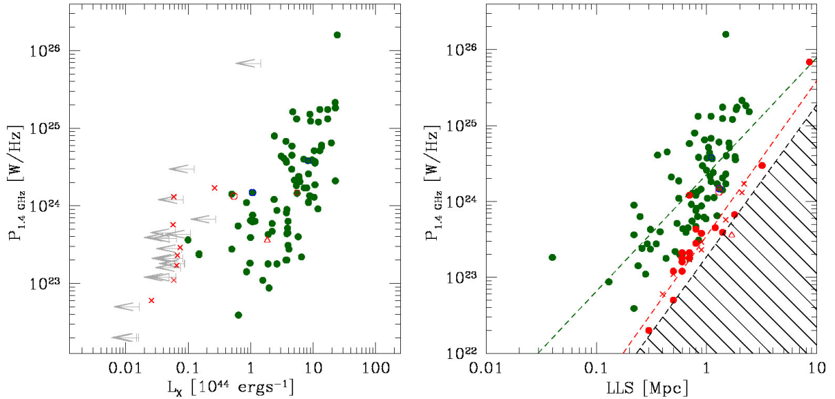
Figure 18. Left panel: Radio power at 1.4 GHz P_{1.4\text{GHz}} versus X-ray luminosity in the energy band 0.1 – 2.4 keV L_{X,0.1-2.4\text{keV}} . Right panel: Radio power P_{1.4\text{GHz}} versus LLS both at 1.4 GHz. Green dots and blue open symbols are from Feretti et al. (2012). Red symbols are measurements from this work: open symbols identify A523 (circle), A520 (square), G4 (triangle), while crosses identify the remaining sources with an X-ray identification. Grey arrows are upper limits from this work. The shaded area in the right panel indicates the region of the (P_{1.4\text{GHz}}, \text{LLS}) plane that cannot be accessed considering the 2\sigma ( \sigma=2.5 mJy/beam) sensitivity of the SRT+NVSS image after point source subtraction. Dashed lines represent a linear fit in logarithmic scale of Eq. 1 for cluster sources (green) and for the new sources (red).
