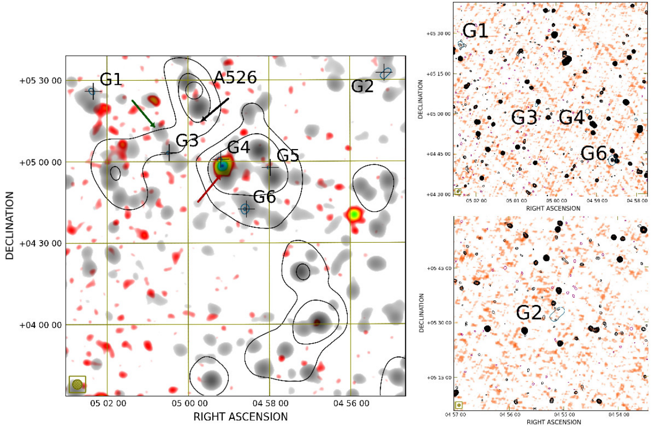
Figure 14. Region G. Left panel: SRT contours ( -60 mJy/beam, 60 mJy/beam, 150 mJy/beam, 500 mJy/beam, negative in magenta and positive in black; resolution 13.9' \times 12.4' ) and SRT+NVSS after compact sources subtraction contours (in blue, starting from 3\sigma and the remaining increasing by a factor \sqrt{2} ; \sigma=2.5 mJy/beam, resolution 3.5' \times 3.5' ) overlaid on X-ray emission from the RASS in red colours and radio emission from the SRT+NVSS (resolution 3.5' ) in gray colours. Right panels: NVSS contours -3\sigma (magenta, \sigma=0.45 mJy/beam), 3\sigma , and increasing by a factor \sqrt{2} (black) overlaid on the TGSS in colours. The black and red arrow mark respectively the locations of the galaxy cluster ZwCl0457.0+0511 and of the compact source PMN J0459+0455, while the green arrow a bridge of radio emission detected by SRT. The colorbars are the same as in Fig. 7.
