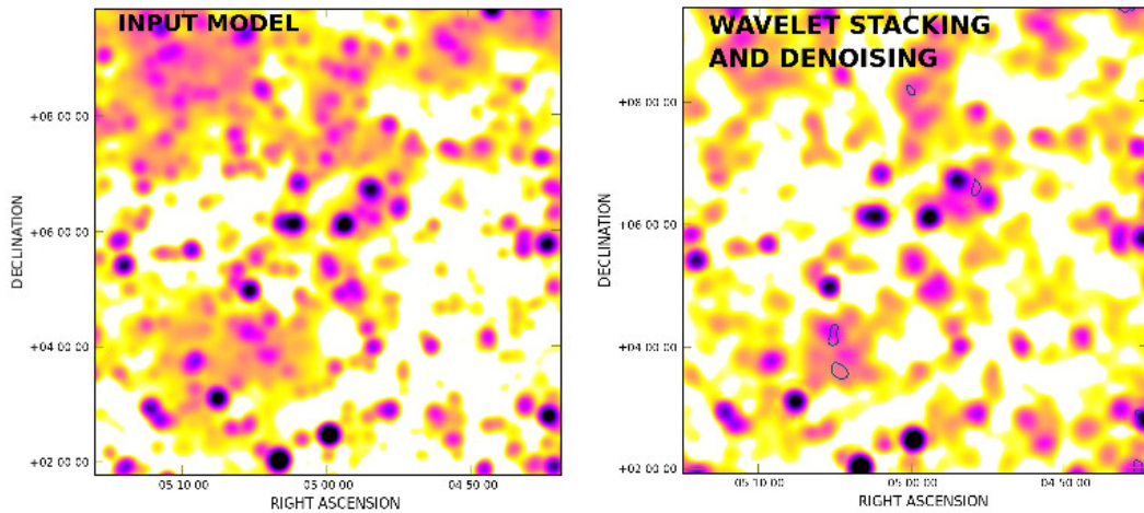
Figure C3. Left panel: model of the sky including the point-like sources and a model of our Galaxy foreground. Right panel: The colours represent the radio emission obtained by applying the imaging pipeline to mock observations including a Galactic and a point-like source contribution. Blue contours show the diffuse synchrotron patches after the NVSS point-like source model has been subtracted and start from 3\sigma of the wavelet stacking and denoising image.
