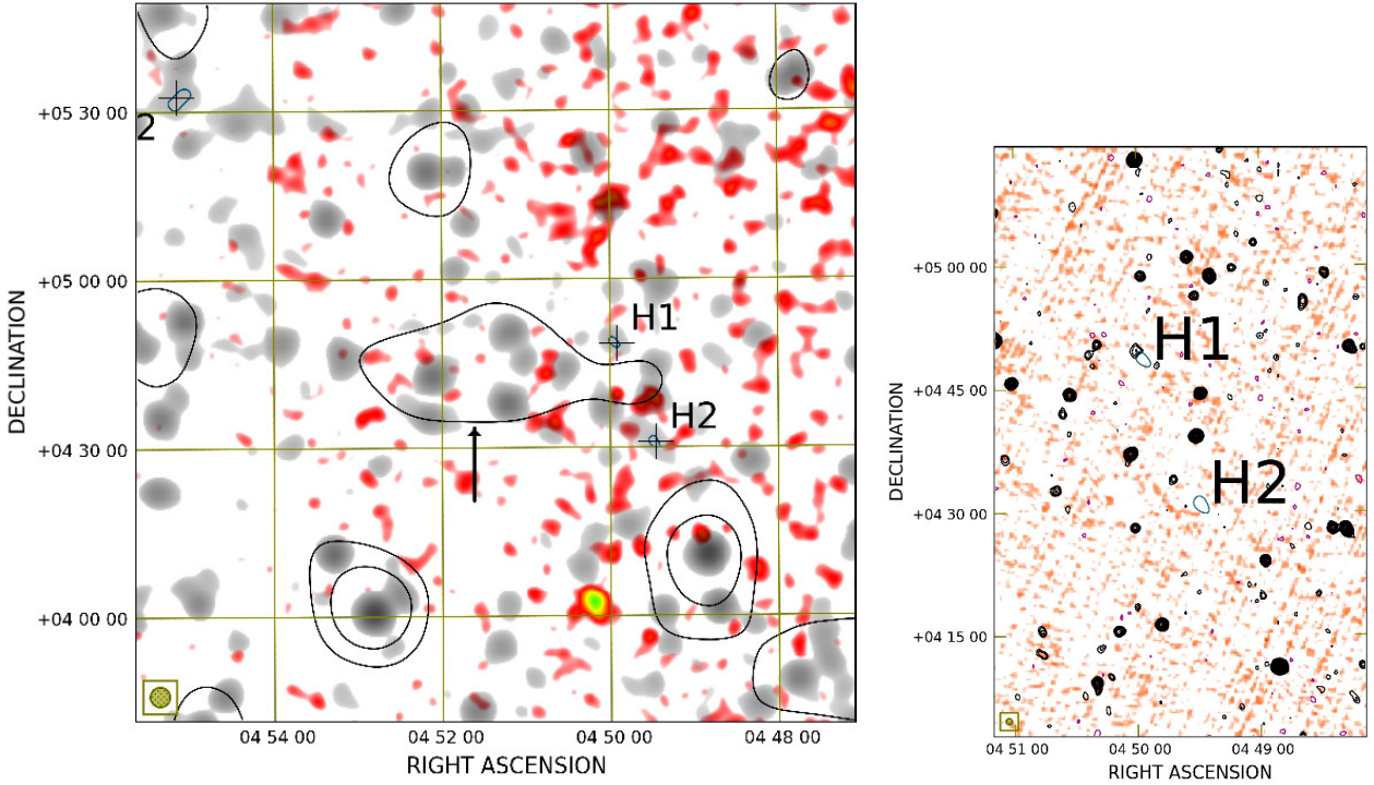
Figure 15. Region H. Left panel: SRT contours ( -60 mJy/beam, 60 mJy/beam, 150 mJy/beam, 500 mJy/beam, negative in magenta and positive in black; resolution 13.9' \times 12.4' ) and SRT+NVSS after compact sources subtraction contours (in blue, starting from 3\sigma and the remaining increasing by a factor \sqrt{2} ; \sigma=2.5 mJy/beam, resolution 3.5' \times 3.5' ) overlaid on X-ray emission from the RASS in red colours and radio emission from the SRT+NVSS (resolution 3.5' ) in gray colours. Right panel: NVSS contours -3\sigma (magenta, \sigma=0.45 mJy/beam), 3\sigma , and increasing by a factor \sqrt{2} (black) overlaid on the TGSS in colours. The black arrow marks a blending of point-like sources. The colorbars are the same as in Fig. 7.
