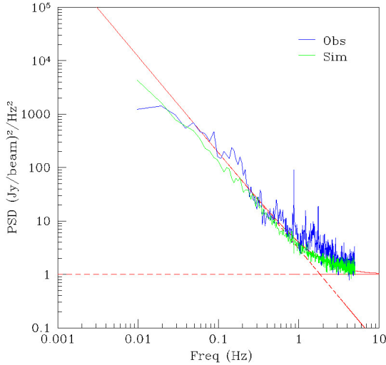
Figure C1. Power spectrum of the noise derived from the observations (blue) and from the simulations (green). The horizontal and diagonal red dashed lines represent respectively the white-noise and 1/f -noise components, while the red continuous line is the sum of white and 1/f -noise.
