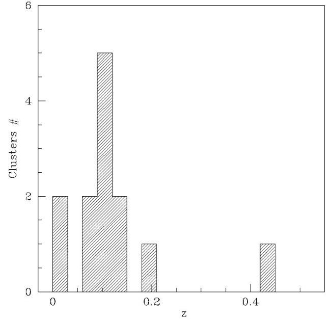
Figure 1. Redshift distribution of clusters in the field of view with a redshift identification.
