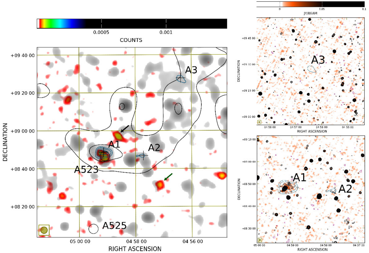
Figure 7. Region A. Left panel: SRT contours ( -60 mJy/beam, 60 mJy/beam, 150 mJy/beam, 500 mJy/beam, negative in magenta and positive in black; resolution 13.9' \times 12.4' ) and SRT+NVSS after compact sources subtraction contours (in blue, starting from 3\sigma and the remaining increasing by a factor \sqrt{2} ; \sigma=2.5 mJy/beam, resolution 3.5' \times 3.5' ) overlaid on X-ray emission from the RASS in red colours and radio emission from the SRT+NVSS (resolution 3.5' ) in gray colours. Right panels: NVSS contours -3\sigma (magenta, \sigma=0.45 mJy/beam), 3\sigma , and increasing by a factor \sqrt{2} (black) overlaid on the TGSS in colours. The black and green arrows mark regions where a strong X-ray emission is detected, as described in the text.
