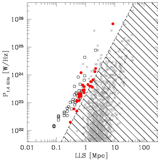
Figure 22. Radio power at 1.4 GHz versus the LLS at 1.4 GHz for the all simulated objects before the SRT observing parameters are considered (gray crosses), for simulated objects after the SRT noise and spatial resolution are applied (empty black dots), and for observed objects (full red dots). The shaded area indicates the region of the (P_{1.4\text{GHz}}, \text{LLS}) plane that cannot be accessed considering the 2\sigma ( \sigma = 2.5 \text{ mJy/beam} ) sensitivity of the SRT+NVSS image after point source subtraction.
