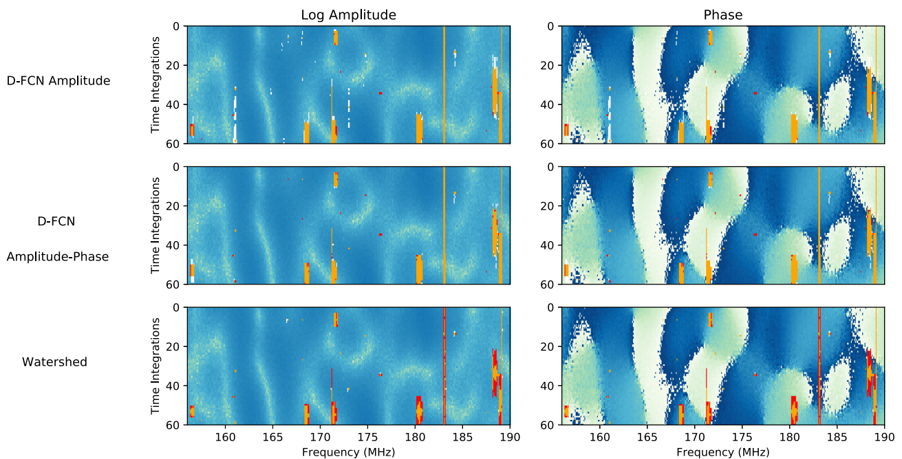
Figure 8. A similar comparison as in Fig. 7 demonstrating how each RFI flagging algorithm performs on simulated HERA data from hera.sim . Orange indicates TP, white is FP, and red is FN. The simulated waterfall visibility is of a 25\lambda baseline dominated by strong diffuse emissions from the de Oliveira-Costa et al. (2008) GSM. The Watershed algorithm’s inability to discriminate between RFI and sky, as indicated by its higher FN rate, in this instance hints that there is required fine-tuning of its kernel size and initial threshold hyperparameters, due to the spectral structure in our simulations.
