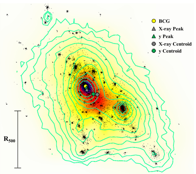
Figure 1. An illustrative example of a combination of the mock multiwavelength maps described in Section 2.2, for the central galaxy cluster at z = 0.46 , in region 85 of the simulation. The y colour map and the contours of the X-ray photon counts, in log scale, are superimposed on the optical SDSS r band. Isocontour levels are logarithmic equispaced by a factor \log 2 . The symbols in the figure mark the position of the relevant cluster centres for the offset parameters, described in Section 4.2. The position of the BCG is marked with a yellow dot, the X-ray and y peaks with a grey and green triangle, and the centroids with crosses, respectively, of the same colours. The R_{500} radius of the cluster is shown in the left-hand corner of the figure.
