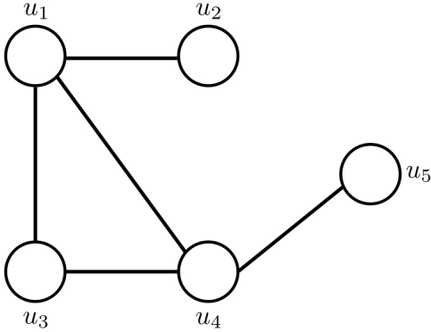
Fig. A.1. Example unweighted graph.
