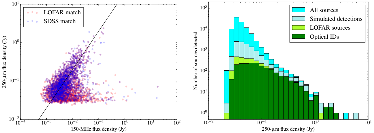
Figure 14. Results of cross-matching Herschel and LOFAR sources. Left: LOFAR/H-ATLAS flux density plot showing positional crossmatches to the LOFAR positions (red) and positions of optical counterparts (blue). Right: detection histogram, showing the distribution of 250- \mu\text{m} flux densities in the whole area-matched sample, the simulated number of detections if S_{150\text{ MHz}} were 0.05 S_{250\text{ }\mu\text{m}} for all sources, the distribution of flux densities of sources matched to LOFAR positions and the distribution for sources matched to SDSS sources. Note the logarithmic axes: at S_{250} < 0.1 Jy fewer than ten per cent of the Herschel sources are detected by LOFAR .
