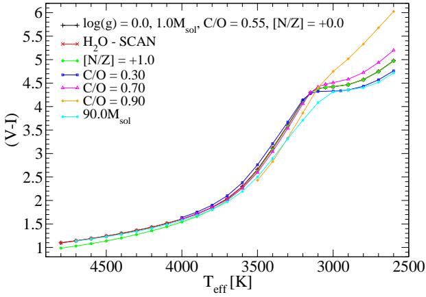
Figure 10. (V-I) as a function of the effective temperature for COMARCS models with solar metallicity and \log(g [cm/s 2 ]) = 0.0. Parameters, symbols and lines are like in Fig. 9.
