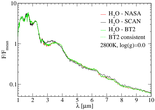
Figure 3. Spectra calculated with different H 2 O data based on a COMARCS model with T_{\text{eff}} = 2800 K, \log(g \text{ [cm/s}^2]) = 0.0 , one solar mass and solar metallicity. The SCAN (black, used in this work as standard), BT2 (green, used in this work as standard) and NASA-AMES (red) line lists are compared. The intensities \nu L_{\nu} are normalized to their mean value. We also show the result obtained with a consistent usage of the BT2 data for the computation of the atmospheric structure and the spectrum (green dashed), which is very similar to the one, where BT2 was only taken for the a posteriori radiative transfer (green full).
