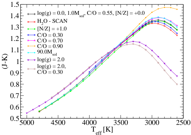
Figure 11. (J-K) as a function of the effective temperature for COMARCS models with solar metallicity. The standard parameters are \log(g [cm/s 2 ]) = 0.0, M/M_{\odot} = 1.0 , solar abundances ( C/O = 0.55 , [N/Z] = 0.0 ) and usage of the BT2 linelist for water below 4000 K (black). The result of changing C/O to 0.3 (blue), 0.7 (magenta) and 0.9 (orange), of increasing nitrogen by a factor of ten ( [N/Z] = +1.0 , green) or the mass to 90 M_{\odot} (cyan) is shown. In addition, we demonstrate the effect of taking the H_2O opacities from the SCAN data (red) and of adopting \log(g [cm/s 2 ]) = 2.0 with C/O = 0.55 (violet) or 0.3 (brown).
