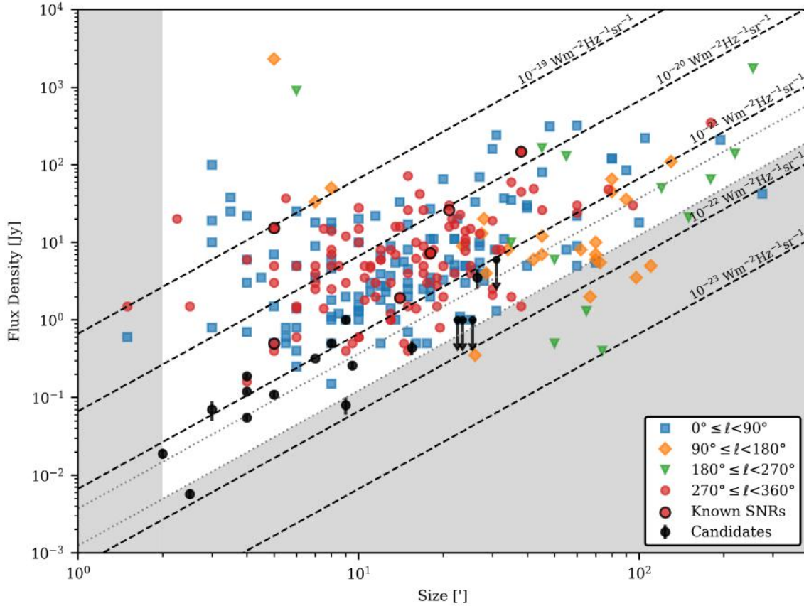
Figure 11. Sizes and flux densities of our SNR candidates compared with the known SNR population as a function of quadrant (data from Green (2022) ), sources without flux estimates omitted). The "Known SNRs" are the six SNRs that are fully imaged in our field. The "Candidates" are the 18 SNR candidates listed in this paper for which we were able to obtain flux estimates. Note that for some candidates the error bars are too small to be visible and others have arrows to indicate that the values should be taken as upper limits. The dashed lines are lines of constant surface brightness. Shaded regions indicate the approximate limits of what we believe we should be able to detect with ASKAP at this frequency. The grey dotted lines represent the \sigma and 3\sigma thermal noise limits.
