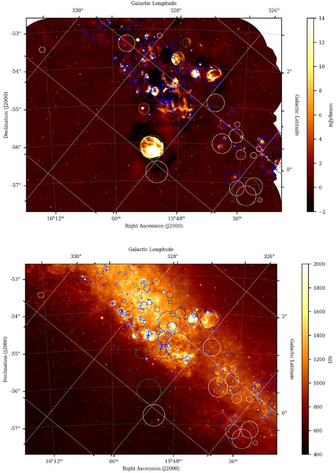
Figure 3. The top image shows the EMU/POSSUM Galactic pilot II field from ASKAP at 933 MHz in total intensity. The bottom image shows the same field in the mid-infrared from WISE (12 \mu m). The green circles show the locations of known SNRs, taken from Green (2022) . The blue circles indicate the locations of known HII regions, taken from Anderson et al. (2014) . The white circles indicate the locations of our SNR candidates.
