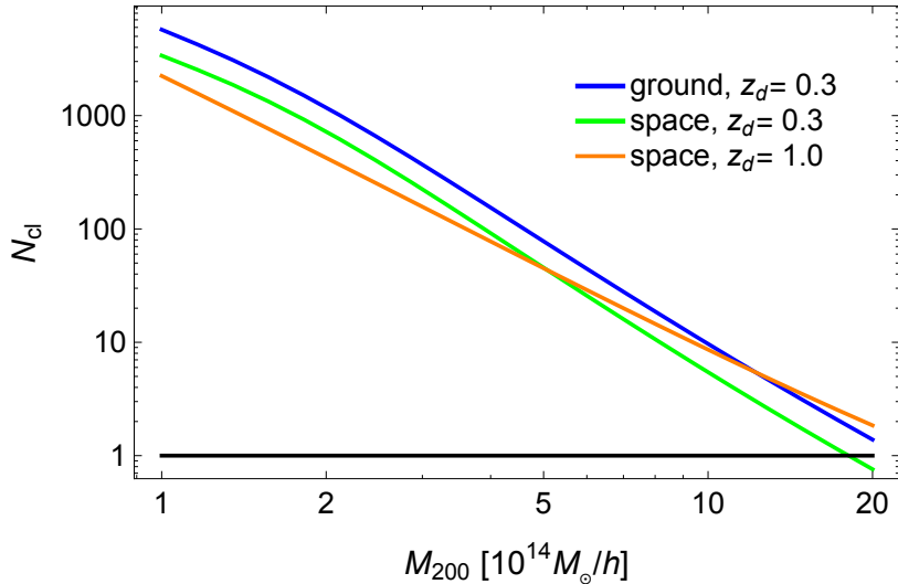
Figure 3. Number N_{\text{cl}} of clusters of mass M_{200} that have to be stacked to distinguish Einasto from NFW shear profiles for different surveys and different lens redshifts z_d .
