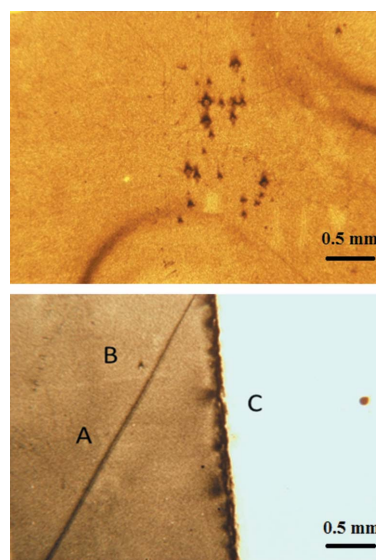
Figure 2 Double-crystal topographs of the ADP sample registered on nuclear emulsion using a Ge 620 monochromator and Cu K\alpha_1 radiation. The contrast is reversed with respect to Fig. 1. (a) 3 × 4 mm area showing a magnification of Fig. 1 with emerging dislocations or inclusions. (b) 3 × 4 mm area near the edge of the crystal, showing a scratch A, an emerging dislocation B and the contrast near the edge of the crystal C.
