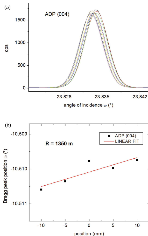
Figure 7 (a) ADP 004 reflectivity profiles spaced 2 mm between adjacent points in a 20 mm range. (b) Bragg peak angular position shift in a 20 mm range of the ADP 004 reflectivity profiles.
