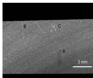
Figure 1 Double-crystal topograph of the ADP sample, registered using an Advacam MiniPIX camera, a Ge 620 monochromator and Cu K\alpha_1 radiation. A: defective pixel; B: tiny scratches due to handling or surface preparation; C: defects, possibly dislocations or crystal inclusions.
