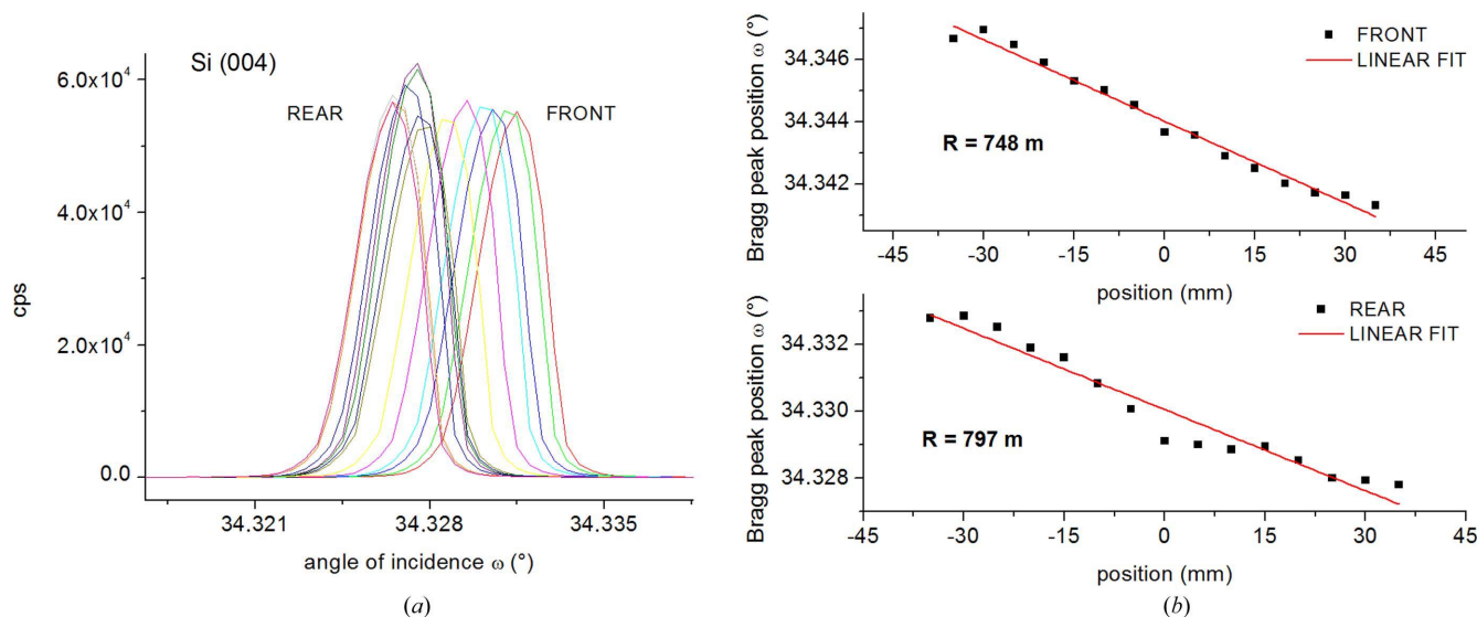
Figure 6 (a) 004 reflectivity profiles taken on both sides of the wafer, with 5 mm spacing between adjacent points in a 70 mm range in a 2 mm-thick perfect silicon crystal. (b) Bragg angle shifts measured on the front and rear surface. The apparent radius of curvature is reported.
