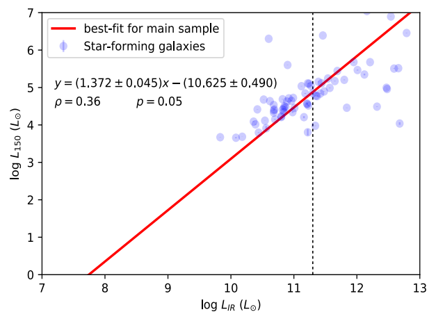
Fig. 10. Top: The correlation between the IR luminosity and the 150-MHz luminosity for the main sample, after excluding AGNs. The vertical dashed line indicates the 90% completeness limit at the median redshift ( z \sim 0.05 ) of the main sample. Bottom: Same as the top panel but for the second sample. The vertical dashed line indicates the 90% completeness limit at the median redshift ( z \sim 0.12 ) of the second sample.
