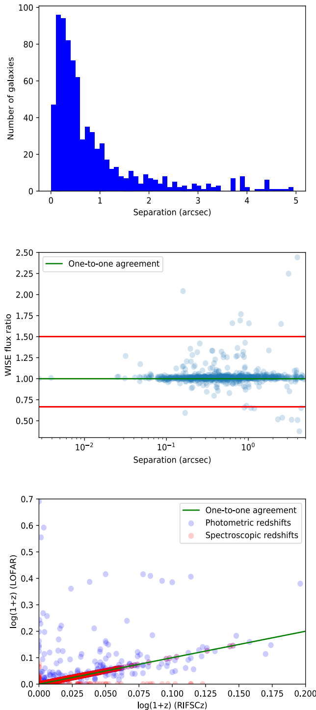
Fig. 1. Top: The distribution of positional separations of sources matched between RIFSCz and LOFAR. Middle: Comparison of WISE W1 flux for sources listed in RIFSCz and in LOFAR. Sources inside the two horizontal red lines have good WISE flux agreement (i.e., the difference is within a factor of 1.5). Bottom: Comparison of redshifts compiled in the RIFSCz and LOFAR VAC.
