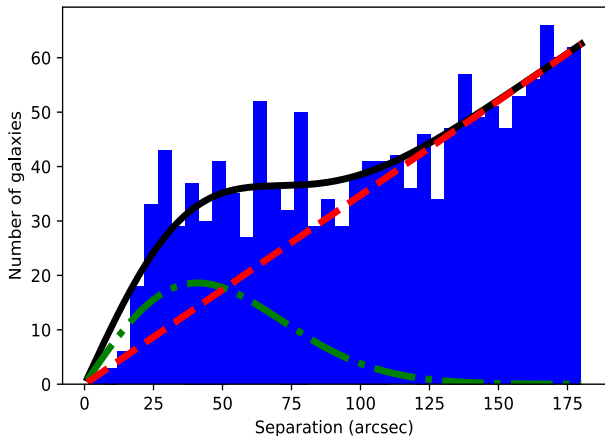
Fig. 2. The distribution of radial offsets between the RIFSCz sources (which only have IRAS observations) and LOFAR sources by selecting all matches within 3' . The radial distribution of the random associations is plotted as the red dashed line, while the radial distribution of the true counterparts is shown as the green dot dashed line. The black solid line is the sum of the two.
