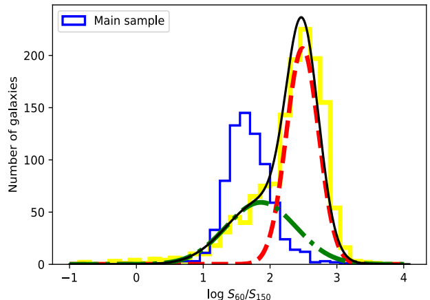
Fig. 3. The 60- \mu m – 150-MHz colour distribution of all matches within 3' between the RIFSCz sources (which only have IRAS observations) and LOFAR sources (yellow histogram). The dot-dashed Gaussian represents the inferred colour distribution of the true counterparts and the dashed Gaussian represents that of the random associations. The black solid line is the sum of the two. The colour distribution of the main sample is shown as the blue histogram.
