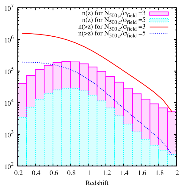
Figure 3. Number of clusters above a given redshift to be detected with overdensities N_{500,c}/\sigma_{\text{field}} > 5 and > 3 in the Euclid photometric survey (dotted blue and solid red lines, respectively). We also show the number density of clusters expected to be detected within redshift bins of width \Delta z = 0.1 for the same detection thresholds (dotted cyan and solid magenta histograms, respectively). The numbers have been obtained by using the reference values of cosmological and nuisance parameters (see Section 4).
