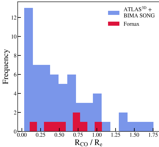
Figure 12. Histogram of R_{\text{CO}}/R_e in the Fornax cluster (crimson) compared to a field sample consisting of gas-rich ETGs from ATLAS 3D (Davis et al. 2013) and spiral galaxies from BIMA SONG (Regan et al. 2001), shown in lilac. Fornax cluster galaxies do not have more significantly truncated CO than the field galaxies (a KS test is not able to reject the null-hypothesis that the Fornax and ATLAS 3D /BIMA SONG samples are drawn from the same distribution, D = 0.29 , p = 0.5\text{--}0.67\sigma ).
