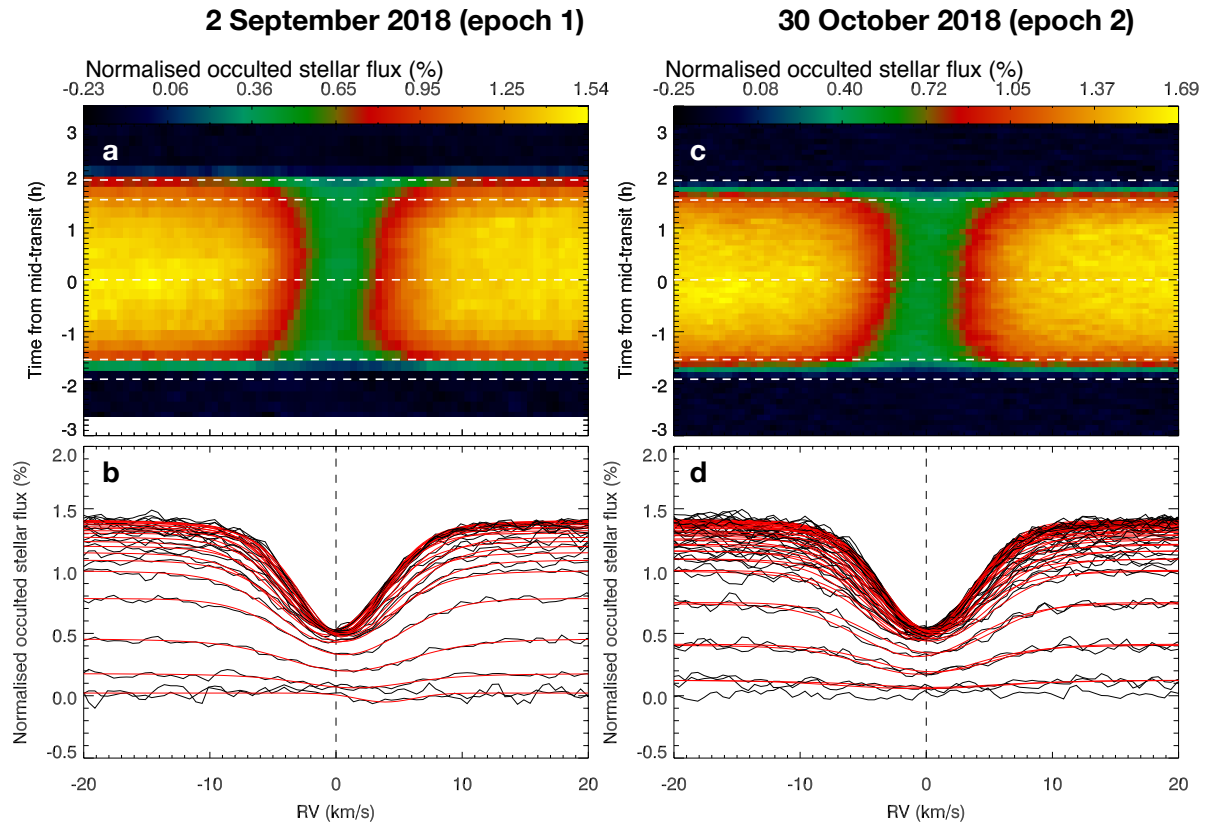
Extended Data Figure 4 | Doppler shadow of WASP-76. a,c, Local stellar CCFs behind the planet represented as a function of time for epoch 1 ( a ) and epoch 2 ( c ). The horizontal dashed lines represent (from bottom to top) the 2 nd contact, mid-transit and 3 rd contact. b,d, 1D view of the local stellar CCFs (black lines) with their Gaussian fits (red curves).
