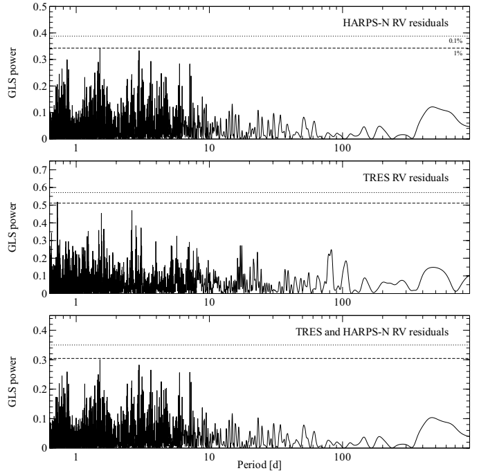
Fig. A.6. GLS periodograms of the RV residuals after subtracting the 2-planets solution and the activity model. In the case of TRES we have included only RVs in the temporal range covered by the activity model, i.e., data gathered since 2013.
