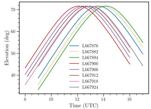
Fig. 1. Elevation plots for the eight observations.
