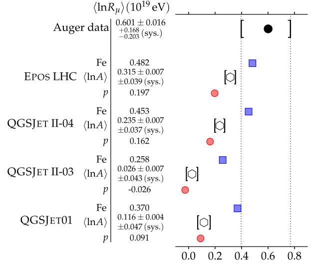
FIG. 6 (color online). Comparison of the mean logarithmic muon content \langle \ln R_\mu \rangle at 10^{19} eV obtained from Auger data with model predictions for proton and iron showers simulated at \theta = 67^\circ , and for such mixed showers with a mean logarithmic mass that matches the mean shower depth \langle X_{\text{max}} \rangle measured by the FD. Brackets indicate systematic uncertainties. Dotted lines show the interval obtained by adding systematic and statistical uncertainties in quadrature. The statistical uncertainties for proton and iron showers are negligible and suppressed for clarity.
