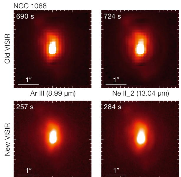
Figure 4. Comparison of images of the active galactic nucleus of NGC 1068 taken with the “old” and the “new” VISIR. After the upgrade, the same quality can be achieved in substantially less time, while having much finer spatial sampling, relevant for all image processing involving deconvolution.
