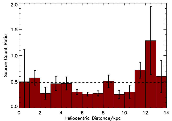
Figure 10. Ratio of the number of YSOs to BGPS clumps as a function of heliocentric distance, with the mean value of 0.49 indicated by the dashed line. The errors are derived using Poissonian statistics.
