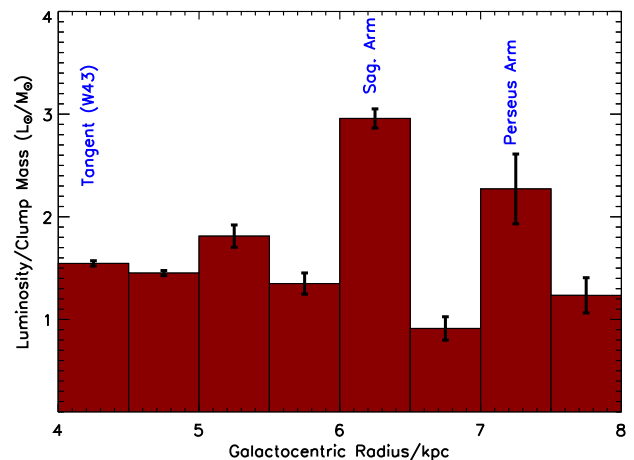
Figure 7. The total L/M as a function of Galactocentric radius within the studied regions centred at l = 30^\circ and 40^\circ . The Galactocentric radii associated with spiral arms are labelled. Sources with heliocentric distances less than 2 kpc are omitted, to remove local sources at Galactocentric radii of \sim 8 kpc.
