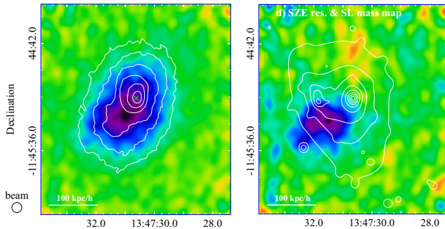
Figure 2: Left : ALMA+ACA image ( \sim 5'' resolution) of RX J1347.5-1145 with X-ray contours overlaid. Right : Substructure in the tSZ effect signal revealed after subtraction of a mean profile excluding the SE quadrant. Lensing contours are overlaid, revealing the location of the dark matter component. Figures from [23].
