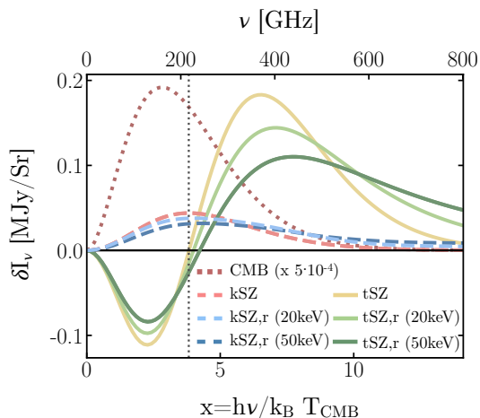
Figure 1: The tSZ (solid) and kSZ (dashed) effects, including relativistic corrections for various electron temperatures. The plots show the SZ effect distortions \delta I_\nu for different scenarios and compositions as a function of (dimensionless) frequency \nu ( x = h\nu/k_B T_{\text{CMB}} ), assuming an optical depth \tau_e = 10^{-2} , a Compton parameter y = 10^{-4} , and a line-of-sight peculiar velocity v_z = +1000 km s ^{-1} (typical of a massive galaxy cluster). The dotted, dark red curve illustrates the Planckian shape of the primary CMB spectrum scaled by a factor of 5 \times 10^{-4} for comparison purposes. Figure from [8].
