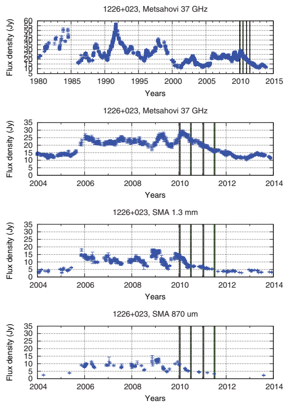
Fig. 9. Flux density curves for 1226+023 at 37 GHz (Metsähovi), 1.3 mm, and 870 \mu\text{m} (SMA). See Fig. 6 for details. Some data come from a dedicated programme by Ann Wehrle.
