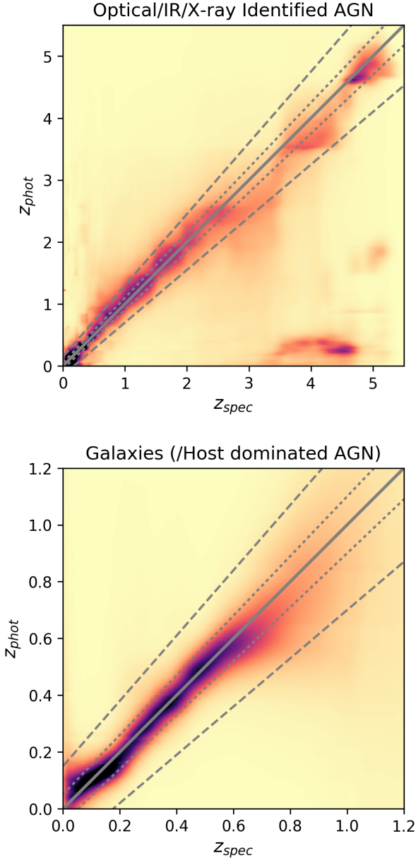
Fig. 12. Stacked probability distributions for the combined AGN selected population ( top panel ; IR, X-ray or optically selected) and the normal galaxy (or host-dominated) population as a function of spectroscopic redshift for the consensus HB photo- z estimate. To improve the visual clarity at higher redshifts where there are few sources within a given spectroscopic redshift bin, the distributions have been smoothed along the x -axis. The solid grey line corresponds to the desired 1:1 relation while the dotted and dashed lines correspond to \pm 0.05 \times (1 + z_{\text{spec}}) and \pm 0.15 \times (1 + z_{\text{spec}}) , respectively.
