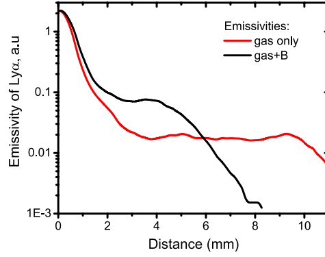
Extended Data Figure 5. X-ray emissivity of Ly \alpha line measured by the FSSR. The red curve represents the piston plasma emission in the range 0–10 mm in the case when the unmagnetized piston expands in the ambient gas. The black curve represents the same but when additionally, the transverse external magnetic field was applied.
