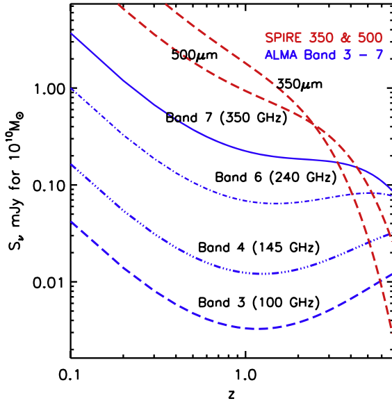
Figure 18. The expected continuum fluxes for the ALMA bands at 100, 145, 240, and 350 GHz and for SPIRE 350 and 500 \mu\text{m} for M_{\text{ISM}} = 10^{10} M_{\odot} derived using the empirical calibration \alpha = 6.7 \times 10^{19} (Scoville et al. 2016) and an emissivity power-law index \beta = 1.8 and including the RJ departure coefficient \Gamma_{\text{RJ}}(25 \text{ K}) . Since the point-source flux sensitivities of ALMA in the four bands are quite similar, the optimum strategy is to use Band 7 out to z \sim 2 –3 above z = 3 . Lower frequency ALMA bands are required to avoid large uncertainties in the RJ correction.
