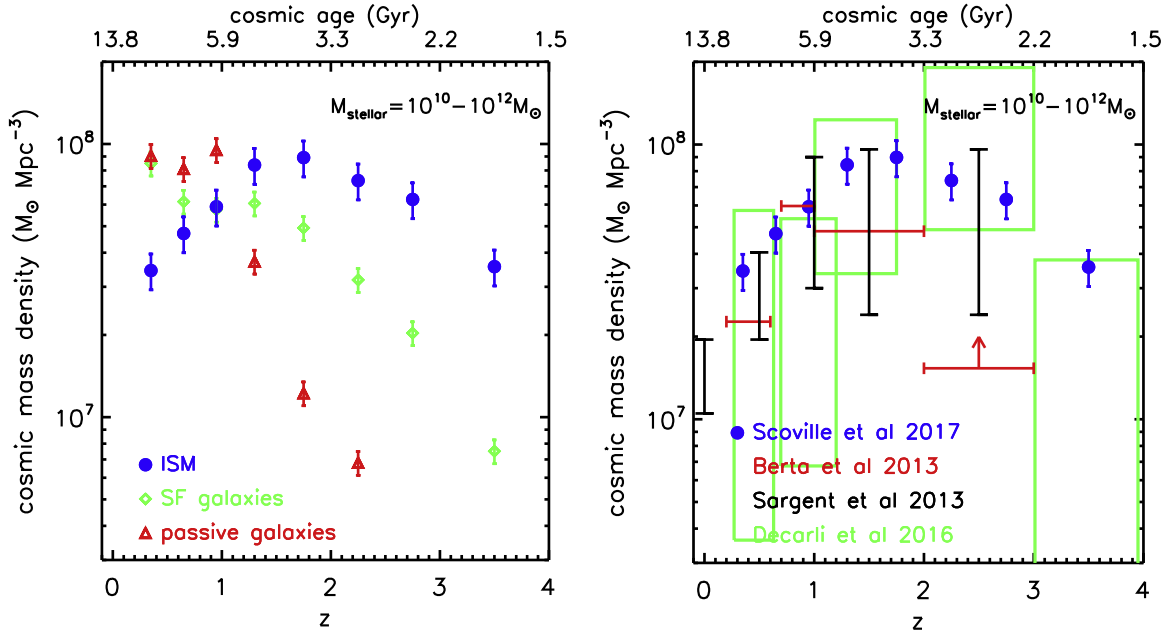
Figure 14. Left: the cosmic evolution of ISM and stellar mass densities in the universe are shown for galaxies with stellar masses M_* = 10^{10} to 10^{12} M_{\odot} . The galaxy stellar mass functions from Ilbert et al. (2013) were used to calculate the ISM masses using Equation (6). Uncertainties in the stellar mass densities are typically \pm 10\% for this range of M_* (see Ilbert et al. 2013, Figure 8); uncertainties in the ISM mass density also include an uncertainty of \pm 10\% in the ISM masses when averaged over the population. (This does not include uncertainty in the calibration of the dust-based mass estimations.) Right: the ISM evolution derived here (blue points) is compared with that obtained by Berta et al. (2013; red horizontal bars and a lower limit), and the ALMA CO survey of Decarli et al. (2016; green boxes) with that derived by theoretical simulation (black vertical error bars; Sargent et al. 2013).
