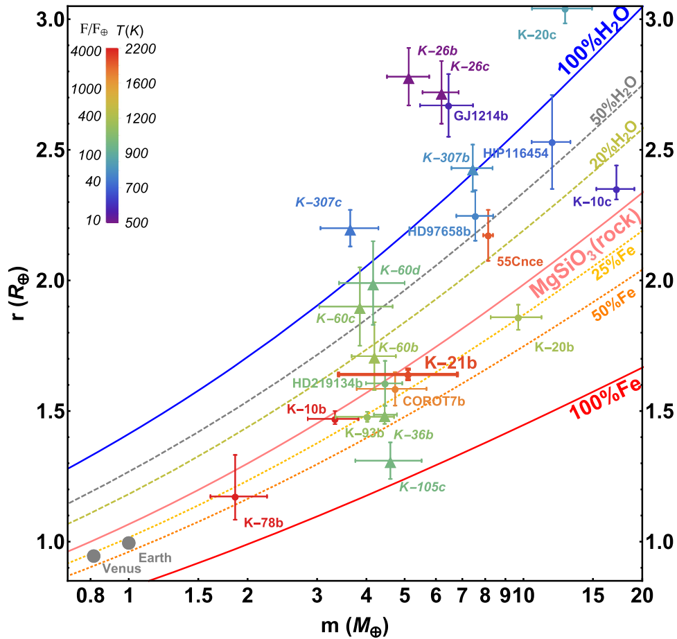
Figure 13. Mass–radius relation for planets with masses < 20 M_{\oplus} , measured with precisions better than 20%. Circles indicate the planets with masses measured via RVs; triangles indicate planets with masses measured via transit timing variations (Carter et al. 2012; Jontof-Hutter et al. 2016). The plot also includes Earth and Venus, for reference. The lines show models of different compositions, with solid lines indicating single composition planets (either \text{H}_2\text{O} , \text{MgSiO}_3 , i.e., rock, or Fe). The dashed and dotted lines indicate Mg-silicate planets with different amounts of \text{H}_2\text{O} and Fe. The data points representing the planets are color coded as a function of incident bolometric stellar flux (compared to the Earth) and equilibrium temperature (assuming circular orbit, uniform planetary surface temperature, and bond albedo A = 0 ). For other A values, the temperature can be obtained by multiplying those values by a factor of (1 - A)^{1/4} , following the flux and temperature scale indicated in the upper-left corner of the diagram.
