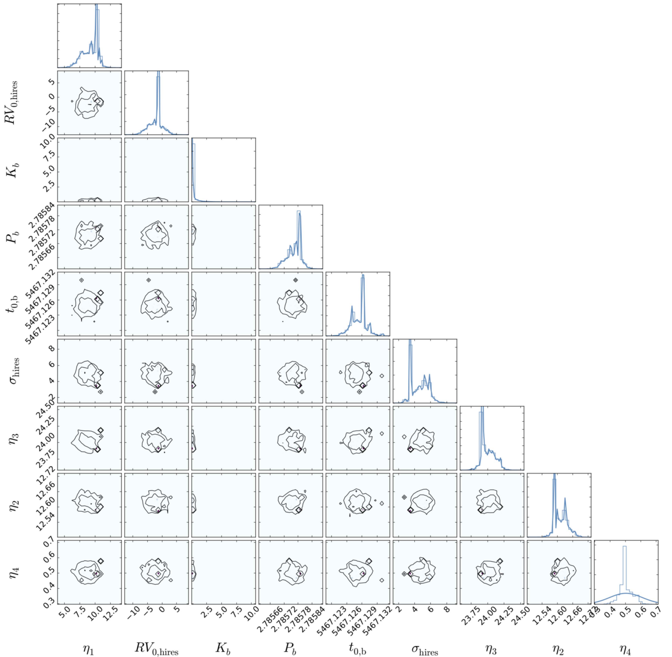
Figure 9. Marginalized 1D and 2D posterior distributions of the model parameters when fitting the HIRES campaign only. The solid lines overplotted on the histograms are kernel density estimations of the marginal distributions. It is clear that the MCMC chain has not converged, despite the additional priors imposed on \eta_1 , RV_{0,hires} , and \sigma_{hires} (the eccentricity was also kept fixed to zero).
