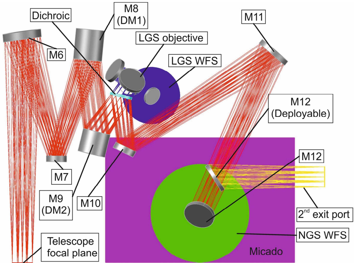
Figure 1. Post Focal Relay optical path.
