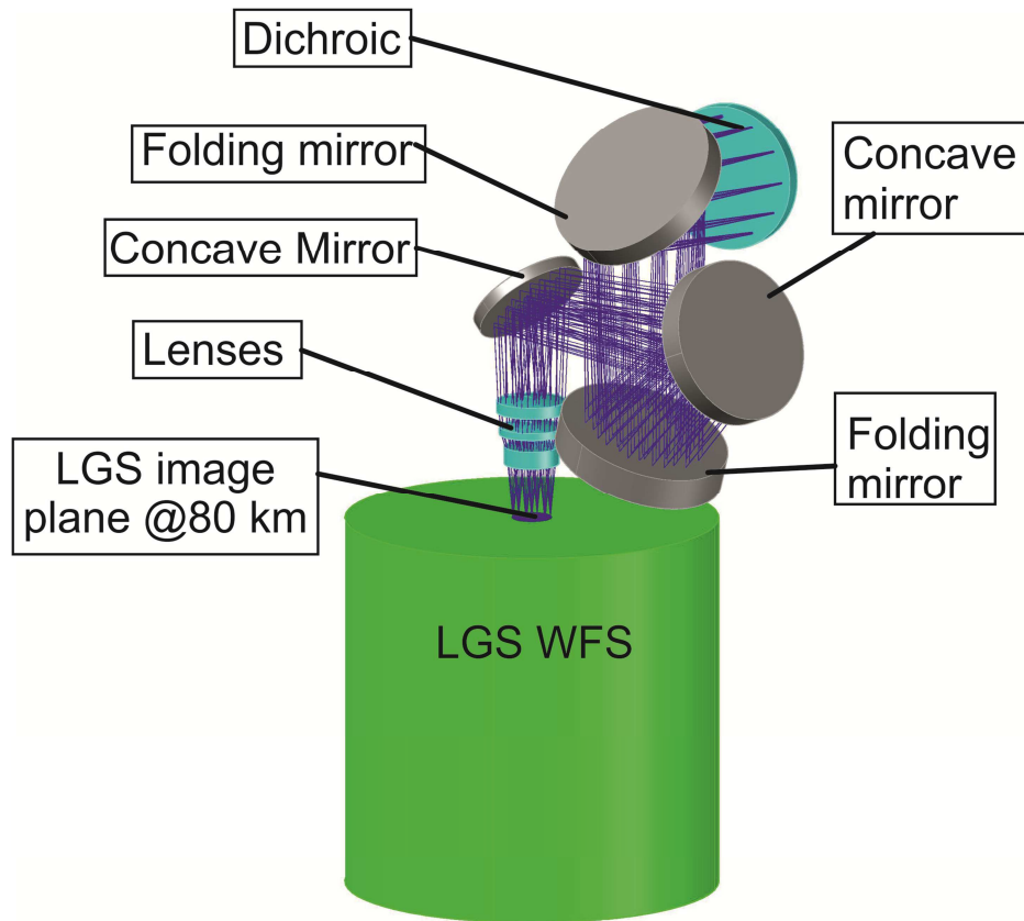
Figure 2. LGS objective. Image plane is kept fixed by the moving lenses that compensate for the source distance variation with the Zenith angle of observation.
