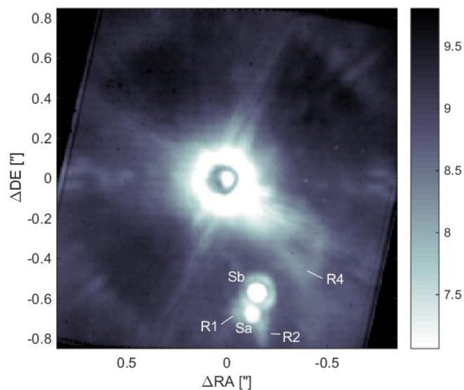
Fig. 4. Coronagraphic H -band (1490–1640 nm) image obtained with the IFS displayed in a logarithmic color scale showing the flux level in magnitude per arcsecond 2 .
