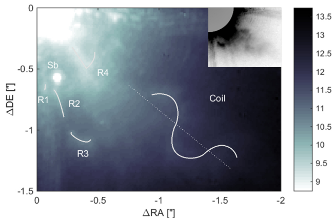
Fig. 2. Zoom on the area southwest of T Tauri N of Fig. 1 showing the coiling structure and the new reflection nebulosity features R1-R4 in the vicinity of T Tauri S. The dashed line connects the inflection points of the coil and points back to the vicinity of T Tauri N. The image tile in the upper right corner shows the same area after subtracting a radial fitted exponential in the outer part of the image to visually enhance the contrast of R3 and the coil.
