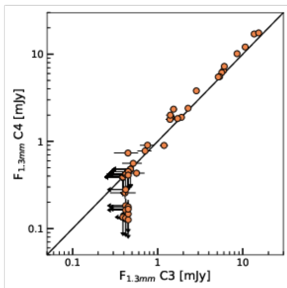
Fig. C.1. Comparison between ALMA fluxes from C3 and C4 for \sigma -Orionis sources. The arrows show 3\sigma upper limits.
