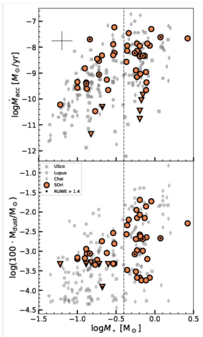
Fig. 4. Top: Mass accretion rates vs stellar mass. The expected uncertainties are indicated by the error bars at the top left. Bottom: Disk masses vs stellar mass. All the targets from our sample and from Rigliaco et al. (2012) are plotted. Downward triangles indicate upper limits. The vertical dashed line indicates a M_* = 0.4 M_\odot .
