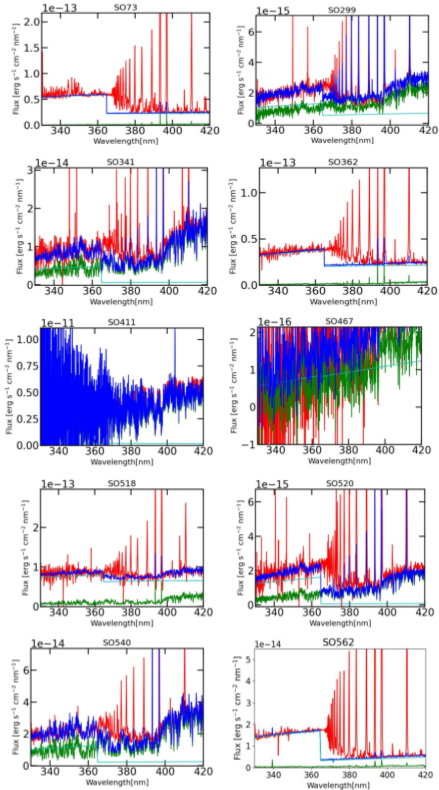
Fig. D.1. Best fit for the Balmer continuum region for targets in the \sigma -Orionis cluster, ordered by source name.
