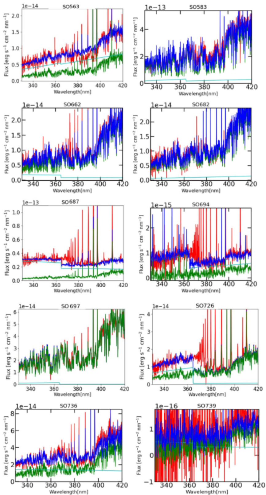
Fig. D.2. Best fit for the Balmer continuum region for targets in the \sigma -Orionis cluster, ordered by source name. - continued
