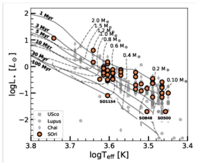
Fig. 2. Hertzsprung-Russell diagram for \sigma -Orionis disks (orange circles) including those from R12. Sources from other SFRs are shown by gray symbols. Isochrones for 1, 3, 5, 10, 30, and 100 Myr from Siess et al. (2000) are overplotted. Evolutionary tracks are from Baraffe et al. (2015).
