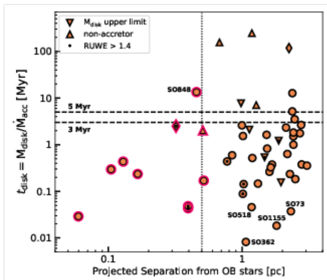
Fig. 7. Distribution of t_{\text{disk}} as a function of projected separation from \sigma -Ori. The triangles indicate the upper/lower limits on \dot{M}_{\text{acc}} and M_{\text{disk}} . The vertical dotted line is located at 0.5 pc from \sigma -Ori. Targets within 0.5 pc are highlighted with an additional red outline. The dashed lines are related to the estimated age of the cluster, i.e. 3-5 Myr (Oliveira et al. 2004).
