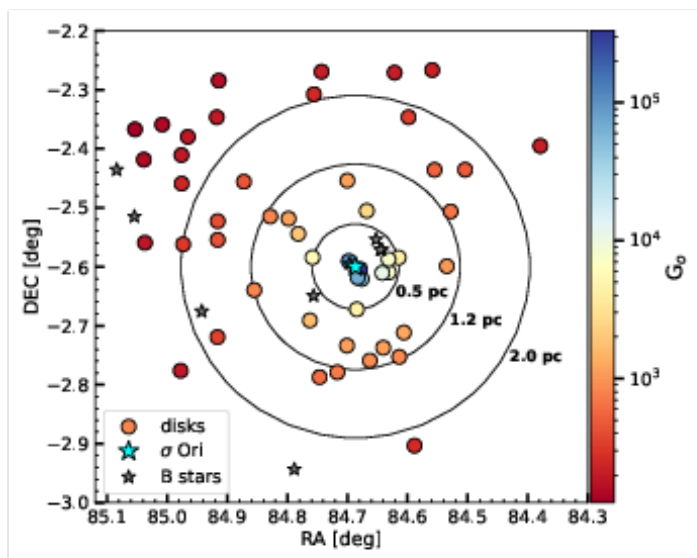
Fig. 1. Spatial distribution of \sigma -Orionis sources (points), and massive O-B stars (star symbols) in the cluster. The massive, multiple system \sigma -Ori is indicated in cyan while the rest of the B-type stars in gray. The color bar shows the incident FUV field strength (in terms of the dimensionless parameter G_0 ) due to the massive stars. Black circles show projected distances of 0.5, 1.2, and 2.0 pc.
