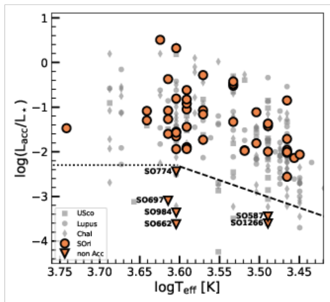
Fig. 3. Ratio between the accretion and stellar luminosities vs effective temperature. \sigma -Orionis sources are indicated by orange circles while stars in other young SFRs by gray symbols. The dotted and dashed lines represent the locus of the chromospheric emission defined by Manara et al. (2013b, 2017a). Downward triangles indicate the non-accretors identified in this work.
