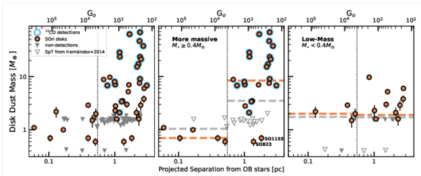
Fig. 5. Disk dust mass ( M_{\text{dust}} ) as a function of projected separation from \sigma -Ori. Left : Considering the whole sample of disks with ALMA observations. Middle : Considering the more massive ( M_{\star} \geq 0.4 M_{\odot} ) stars in our \sigma Orionis sample. Right : Considering the less massive ones ( M_{\star} < 0.4 M_{\odot} ). Dashed lines show the M_{\text{dust}} median inside and outside 0.5 pc for our X-Shooter sample (orange) and also including upper limits with reported SpT in Hernández et al. (2014) (gray). Orange points are continuum detections, downward triangles are 3\sigma upper limits and, ^{12}\text{CO} detections ( 3\sigma ) are indicated by an additional blue circle. The ^{12}\text{CO} fluxes are listed in Table 2 .
