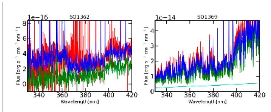
Fig. D.5. Best fit for the Balmer continuum region for targets in the \sigma -Orionis cluster, ordered by source name. - continued
