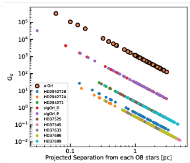
Fig. A.1. G_0 of O and B stars in the \sigma Orionis cluster. The FUV radiation is dominated by the central system \sigma -Ori.
