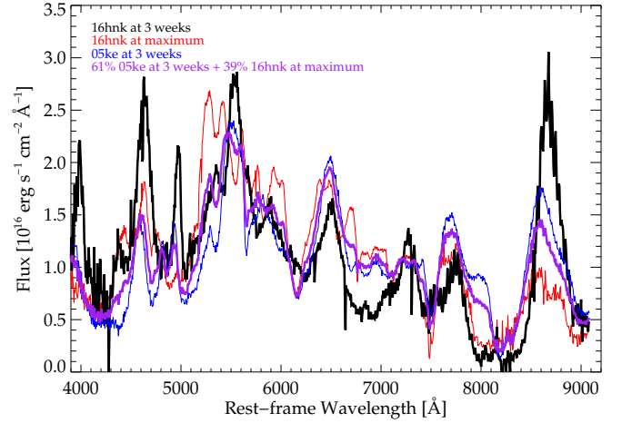
Fig. A.5. Simulation of a LE contaminated spectrum at three weeks past maximum, based on a fiducial subluminous spectrum at +3 weeks past maximum from SN 2005ke (contributing 61% to the total), and adding 39% of the SN 2016hkn spectrum at maximum light, which represents the contamination from the LE. Comparing this LE-affected spectrum (in purple) to the observed SN 2016hkn (in black) we do not see any feature that definitely confirms that the latter is affected by any feature reflected from earlier epochs.
