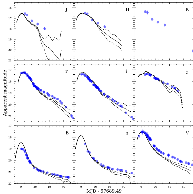
Fig. A.4. Multiband SN 2016hkn SNOOPY fits using a 91bg template and with a 10% contribution of a LE starting at +15 days until the end of the light curve. Fits in all band are reasonably better than those without a LE shown in Fig. 7.
