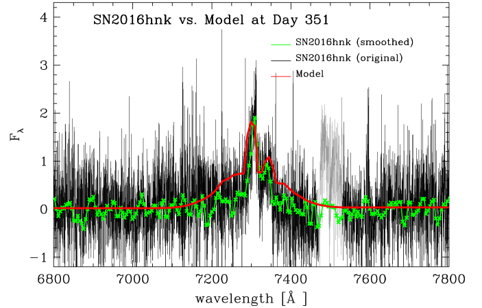
Fig. 27. Comparison of the nebular spectrum of SN 2016hnk with our high-density delayed-detonation model in the rest frame assuming a redshift of z = 0.01610 . The flux is in 10^{-18} \text{ erg s}^{-1} \text{ cm}^{-2} on the same scale as Fig. 19. The telluric region in the original spectrum is plotted in gray, around 7500 \text{ \AA} . The theoretical spectrum is dominated by a narrow, forbidden [Ca II] doublet at 7291 and 7324 \text{ \AA} above a quasi-continuum at about the 3% level formed by many transitions of mostly heavier elements including Fe, Co, Ni, and Cr.
