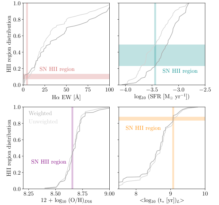
Fig. 5. Top: similar to Fig. 4, the spectrum of the SN 2016hbk parent HII region (blue) and best SSP fit from STARLIGHT (red) are shown. Right panels: stellar subtracted spectra around the H \alpha and H \beta wavelengths. Bottom rows: distributions of the gas-based parameters of all 56 HII regions in MCG -01-06-070, weighted by the contribution of the region to the total SFR of the galaxy (dark lines) or unweighted (light lines). In this case, colored horizontal bands represent the band where the SN 2016hbk parent HII region lies within.
