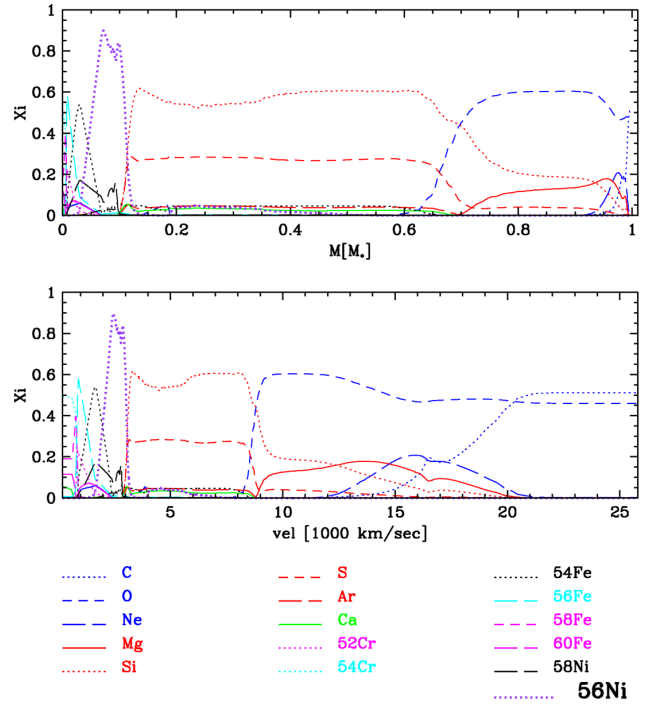
Fig. 25. Same as Fig. 24 but showing the overall abundance structure at large times as a function of mass coordinate ( top ) and expansion velocity ( bottom ). It is very similar to the subluminous model for SN 1999by and consistent with the chemical structure based on our abundance tomography given in Table 3. In addition, we show the initial ^{56}\text{Ni} \rightarrow ^{56}\text{Co} \rightarrow ^{56}\text{Fe} at the time of the explosion (purple dotted line).
