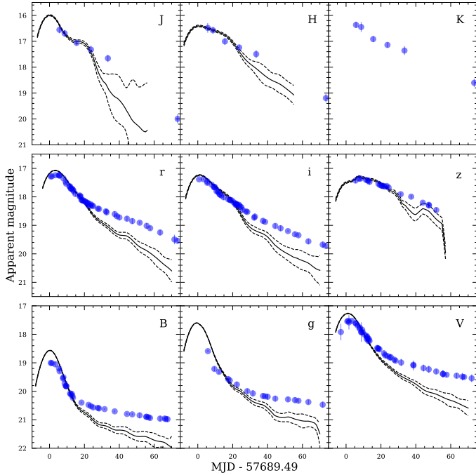
Fig. 7. Multiband light curves of SN 2016hnk (filled circles) compared with a 1991bg-like template (lines). Best-fit SNOOPY parameters are R_V = 2.1 and a host-galaxy color excess of E(B - V)_{\text{host}} = 0.55 mag. We note that beyond +20 d the template fit does not succeed in capturing the SN brightness.
