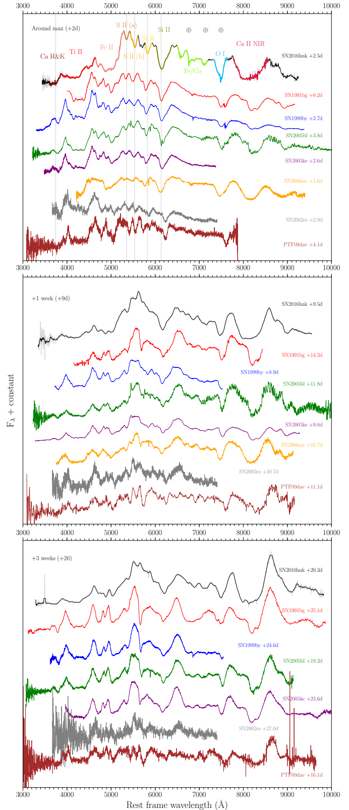
Fig. 14. Spectra of SN 2016hnk at three different epochs (around maximum, after a week, and around three weeks past maximum light) compared to other subluminescent 1991bg-like SNe Ia, PTF09dav (Ca-rich), and SN 2002es (2002es-like SN Ia). The main typical features of 1991bg-like SNe Ia are identified in the top panel . Vertical lines in the top panel are located at the minima of a few features and serve as a comparison of the velocities with respect other objects. All spectra have been Milky Way extinction-corrected and shifted to the rest frame.
