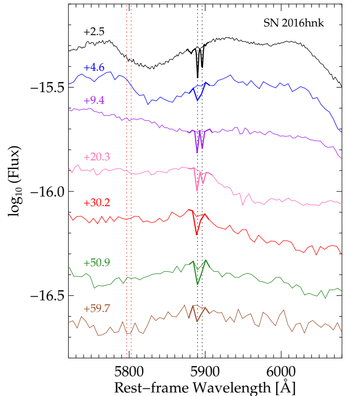
Fig. A.2. Zoom into SN 2016hnk spectra around the Na I D doublet (rest-frame 5890 and 5896 \text{ \AA} ; in vertical black dotted lines) absorption, at seven epochs from +2.5 to +59.7 days after maximum. Thick lines represent Na I D absorption with pEW = 1.3 \text{ \AA} at the spectral resolution of each spectrum. Red vertical lines indicate the position where the Na I D doublet from the Milky Way should be found. In all cases, we do not detect the Na I D lines in SN 2016hnk spectra.
