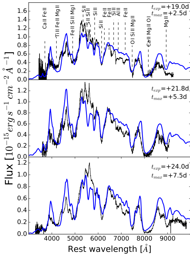
Fig. 21. Time series of data (black) and spectral models (blue) for SN 2016hnk during the photospheric phase. The data were corrected for foreground and host galaxy extinction. The observer-frame time from B -band maximum and the rest-frame time from explosion is provided for each model. Line identifications from the model are shown in the top plot.
