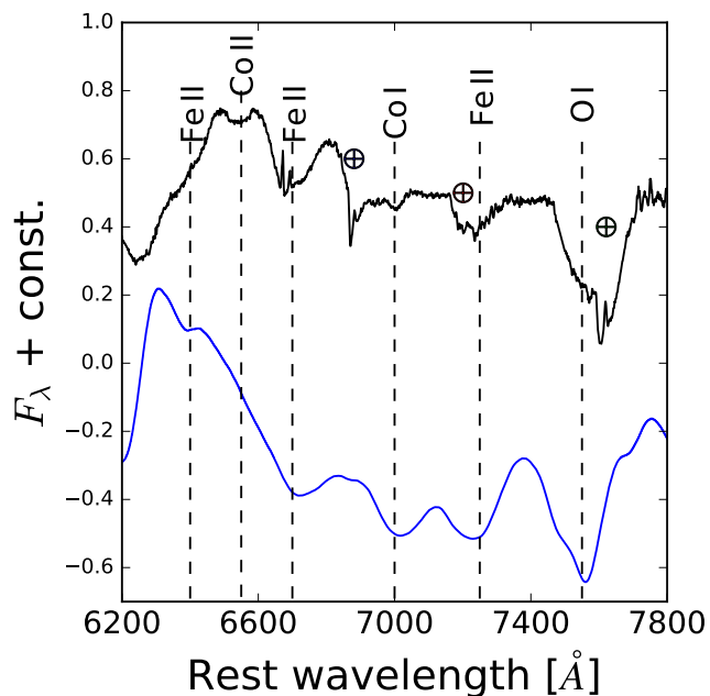
Fig. 23. Comparison of SN 2016hnk (black) +2.5 d past maximum light and the non-LTE model of SN 1999by at +7 days past maximum light (blue) from Höflich et al. (2002). The telluric features are denoted in the observed spectra.
