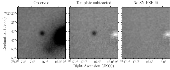
Fig. 2. g -band imaging of SN 2016hnk and its host galaxy, before ( left ) and after ( middle ) subtracting the host galaxy template using hotpants integration in SNOOPY. This example shows how the subtracted image is clean enough to perform PSF fitting, as shown in the right panel where the SN PSF has been removed. A small residual of the galaxy core is shown on the middle and right panels (white blob), however it does not affect SN PSF fitting.
