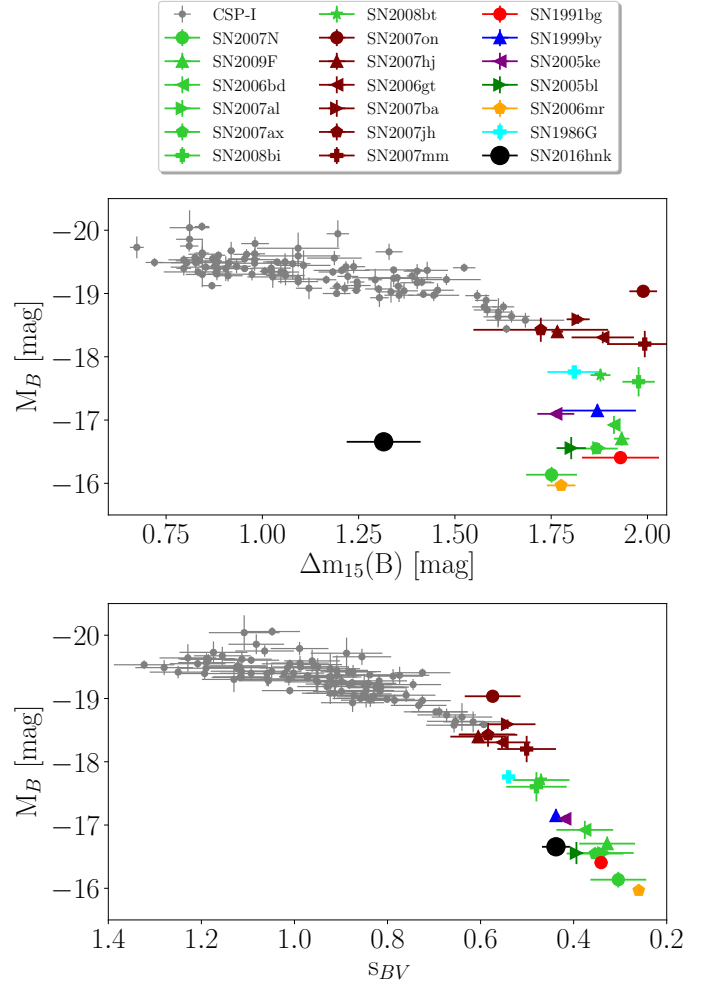
Fig. 10. Luminosity width relation as a function of \Delta m_{15}(B) (top) and s_{BV} (bottom) for a selection of CSP-I SNe Ia from Krisciunas et al. (2017) with the addition of SN 2016hnk (black circle). We note that SN 2016hnk sits off the \Delta m_{15}(B) - M_B relationship because of the degeneracy in \Delta m_{15}(B) for fast declining SNe Ia.
