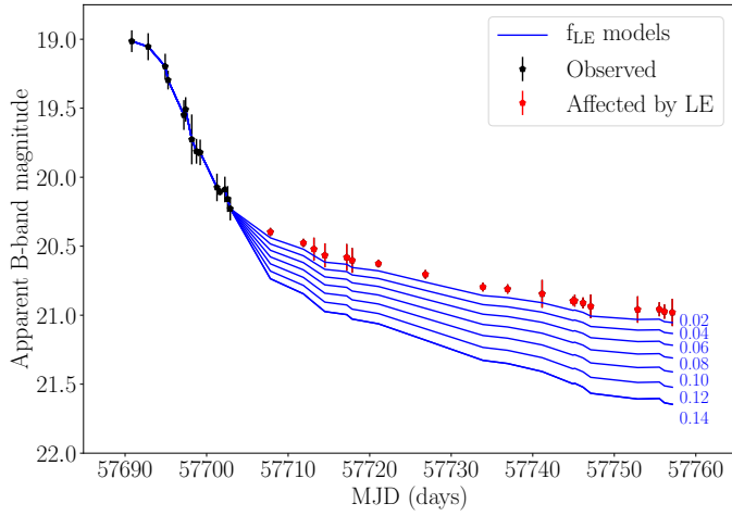
Fig. A.3. Effect of subtracting different fractional contribution of the LE to the SN 2016hkn B band observed light curve.
