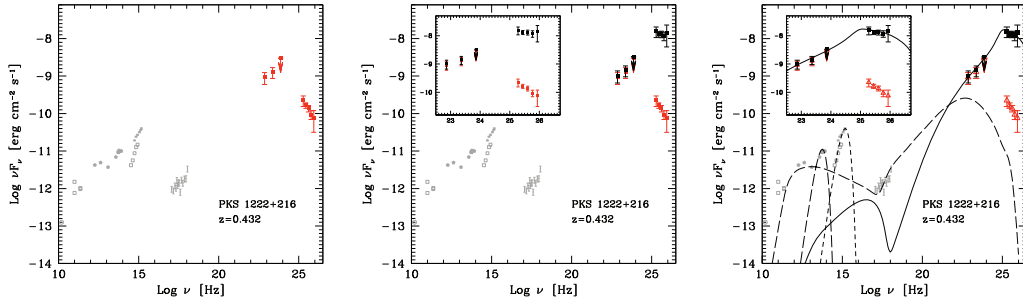
Fig. 1. – Left panel: red triangles at high and VHE are the spectrum of PKS 1222+216 recorded by Fermi /LAT and the one detected by MAGIC but EBL-deabsorbed according to conventional physics. Central panel: red triangles are the same as before, while black squares represent the same data once further corrected for the photon-ALP oscillation effect. Right panel: red triangles and black squares are the same as before, whereas the solid black line is the SED of our model (the other points and broken lines should be presently ignored).
