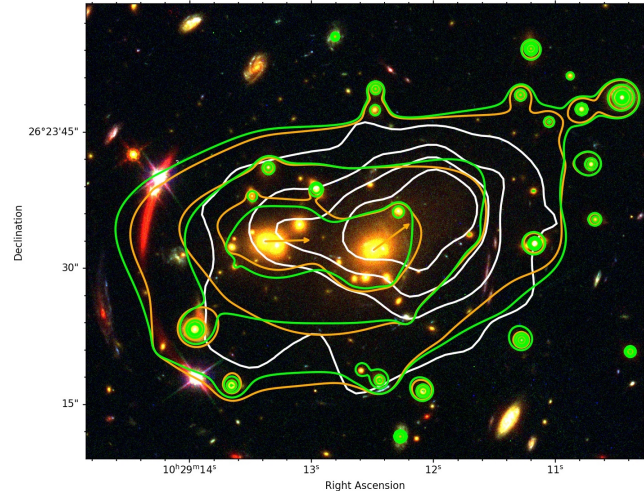
Figure 8. Color composite image of the central region of SDSS1029, where we compare the contour levels of the total surface mass density distribution and the Chandra X-ray surface brightness (in white, after masking the strong emission from the three QSO images). Orange and green contours correspond, respectively, to the best-fit Models 1 and 2 and the levels are [1.0, 1.5, 2.5] \times 10^9 M_{\odot} \text{ kpc}^{-2} . The orange arrows indicate the orientation of the large-scale DM halos in Model 1.
