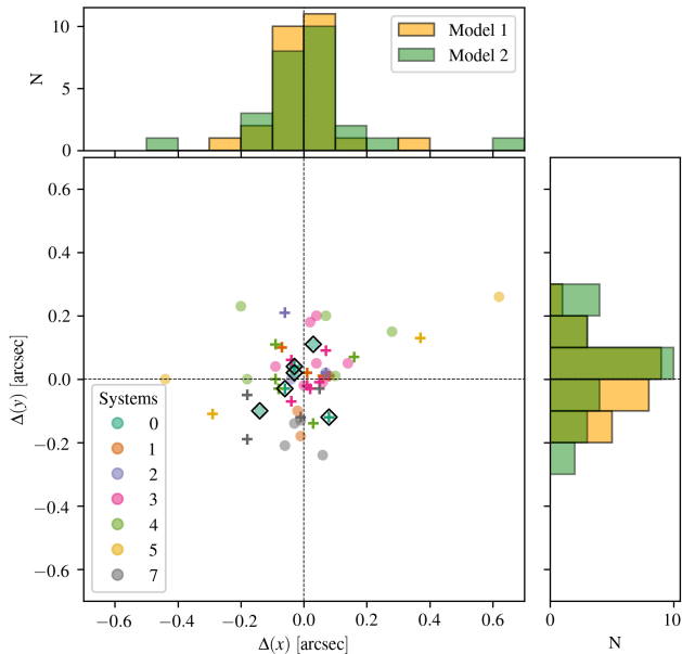
Figure 6. The middle panel shows the distribution of the separations \Delta(x) and \Delta(y) between the observed and model-predicted image positions as crosses(circles) for Model 1(2). Each system is color-coded as in Figure 3. The separations for the quasar images are, in addition, highlighted with black diamonds. The upper and right panels show the marginalized distributions of the \Delta(x) and \Delta(y) separations, respectively.
