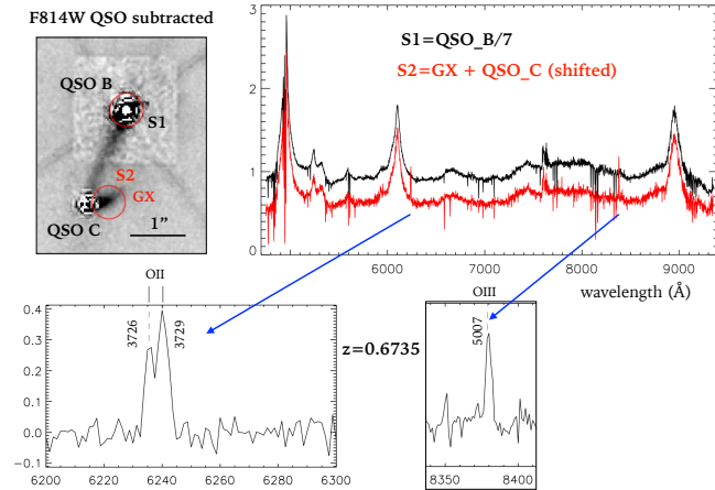
Figure 4. Top: MUSE 1D spectra of the quasar (QSO) image B (S1 in black, rescaled by a factor of 7) and the hidden galaxy GX lying close to it, highly contaminated by the QSO image C (S2 in red). Both spectra are extracted from circular apertures of 0''.3 radius, indicated in red in the HST F814W image cutout, where QSO B and C have been subtracted. Bottom: Two portions of the subtracted 1D spectrum (S2–S1), where the [O II] and [O III] emission lines of a source at a redshift of 0.6735 are highlighted.
