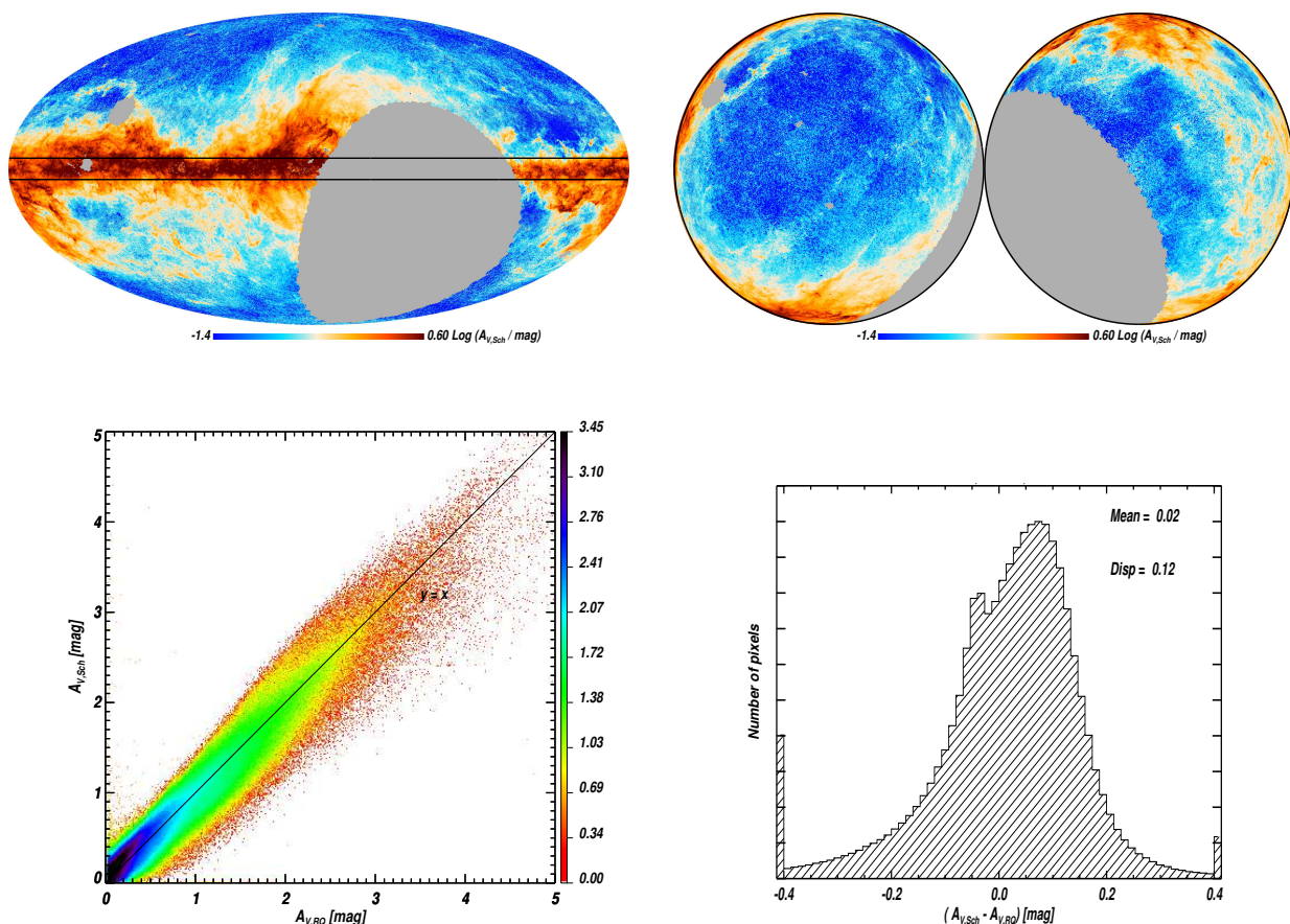
Fig. 10. Comparison between the renormalized DL A_V estimates ( A_{V,RO} ), and those derived from optical stellar observations ( A_{V,Sch} ). The top row shows the A_V maps derived from optical stellar observations. The b = \pm 5^\circ lines have been added for reference. The bottom row left panel compares the renormalized A_{V,RO} estimates with those derived from optical stellar observations A_{V,Sch} in the |b| > 5^\circ sky. The agreement of these independent A_V estimates is a successful test of our empirical renormalization. The bottom row right panel show the histogram of the difference of the two A_V estimates, also in the |b| > 5^\circ sky.
