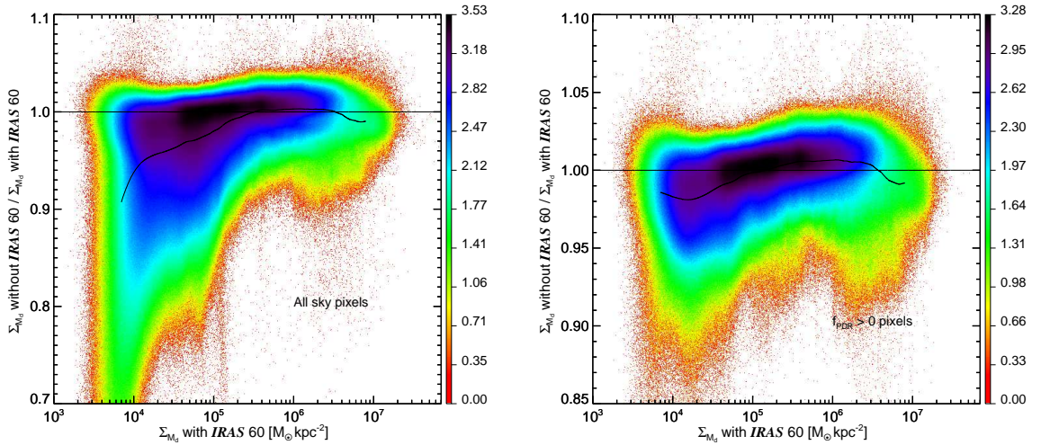
Fig. 6. Comparison between the dust mass estimates when the IRAS 60 constraint is excluded or included in the fit. The left panel shows all the sky pixels, and the right panel only the f_{\text{PDRE}} > 0 pixels. The vertical axis corresponds to the ratio of the inferred mass density of a fit without using the IRAS 60 constraint to that obtained when this constraint is present (see text). Colour corresponds to the logarithm of the density of points (see Fig. 5). The curve corresponds to the mean value.
