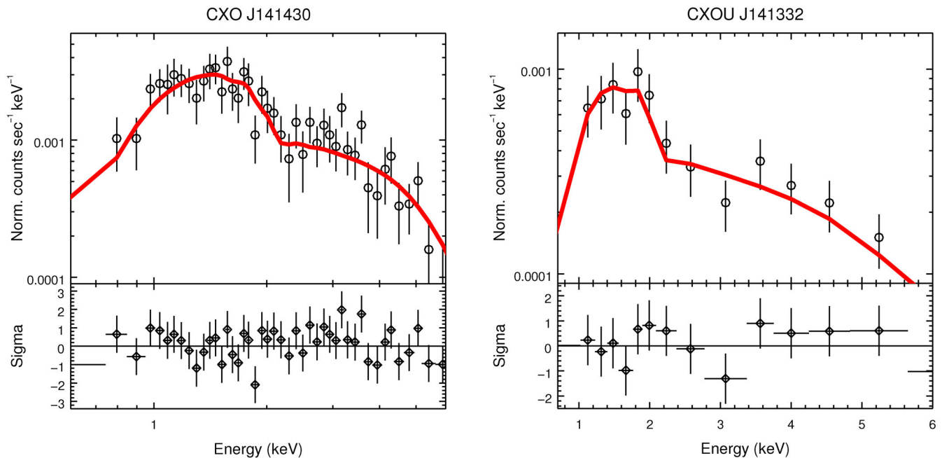
Figure 4. Chandra /ACIS spectra and best-fitting power-law models (red solid line) for CXO J141430 and CXOU J141332 (as indicated in each panel) from observation 12823. Bottom panels: residuals in units of standard deviations.
